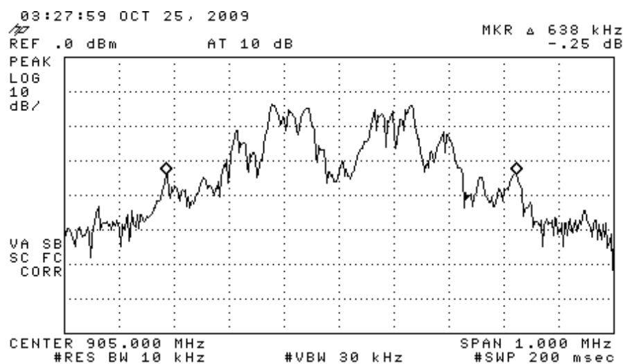
Figure 6.3. Measured emission bandwidth of the DUT (pulsed).
