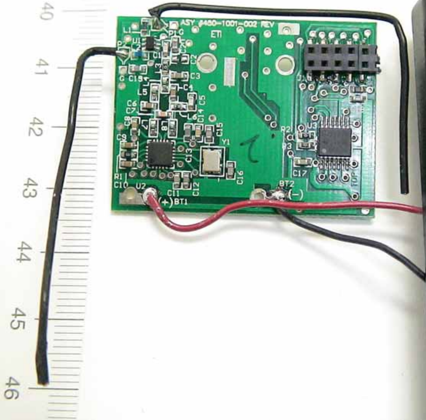
PCB (top)
