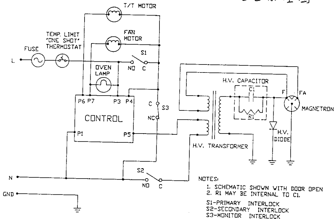
ELECTRICAL SCHEMATIC
