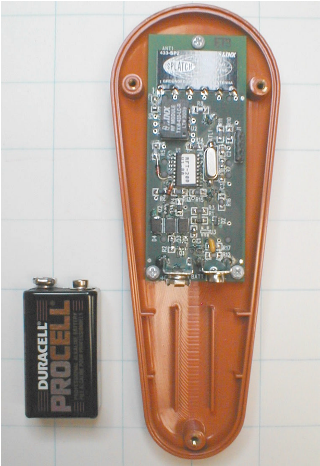
Battery Removed
