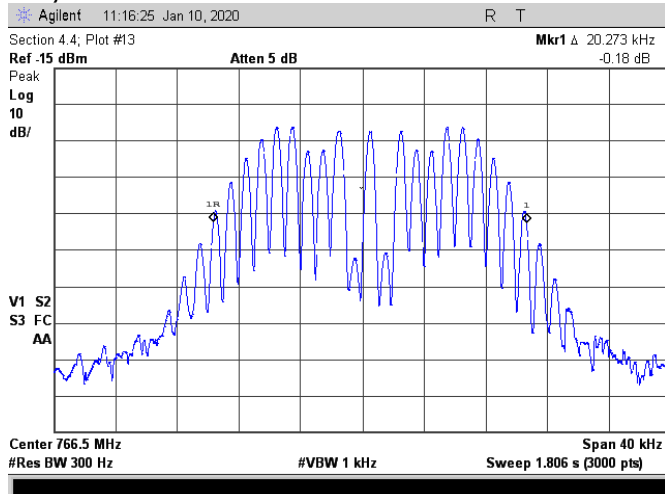
Input Signal to Amp; FM 16K
