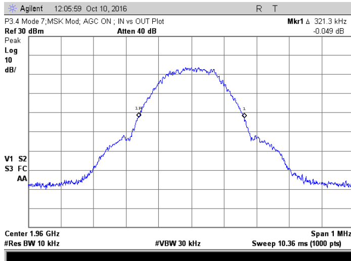
Amp output with AGC; 1.96 GHz, MSK
