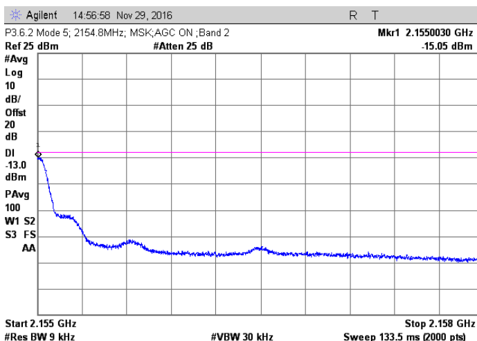
MSK; 2154.8 MHz Injected Signal; AGC on
