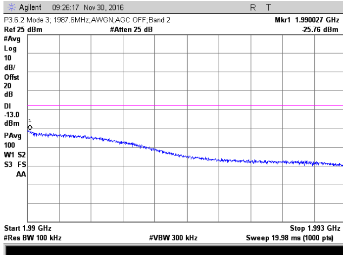
AWGN; 1987.6 MHz Injected Signal; AGC off
