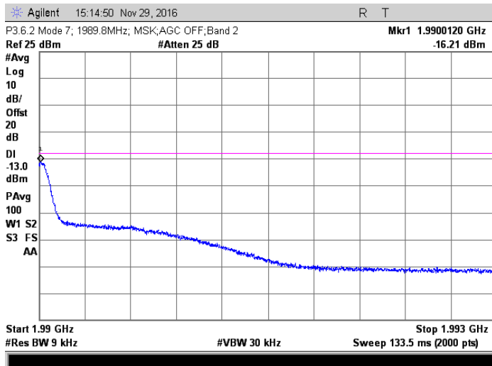
MSK; 1989.8 MHz Injected Signal; AGC off
