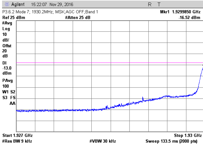
MSK; 1930.2 MHz Injected Signal; AGC off
