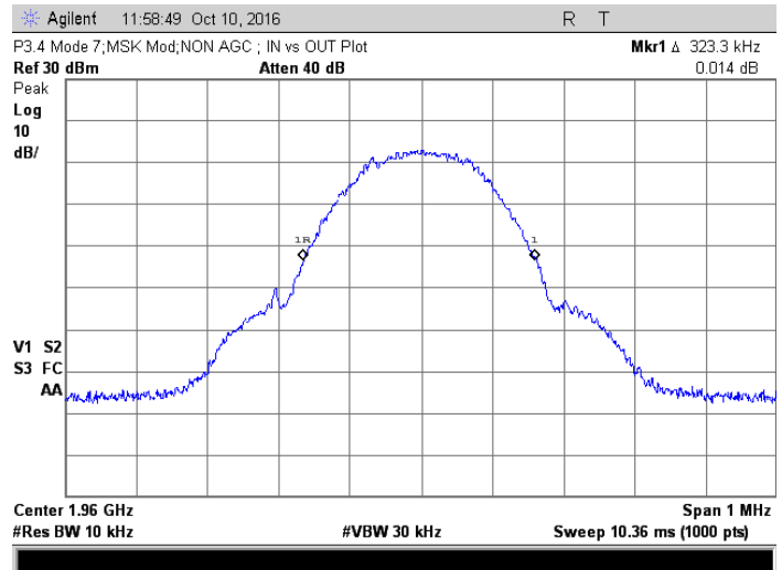
Amp output, no AGC; 1.96 GHz, MSK
