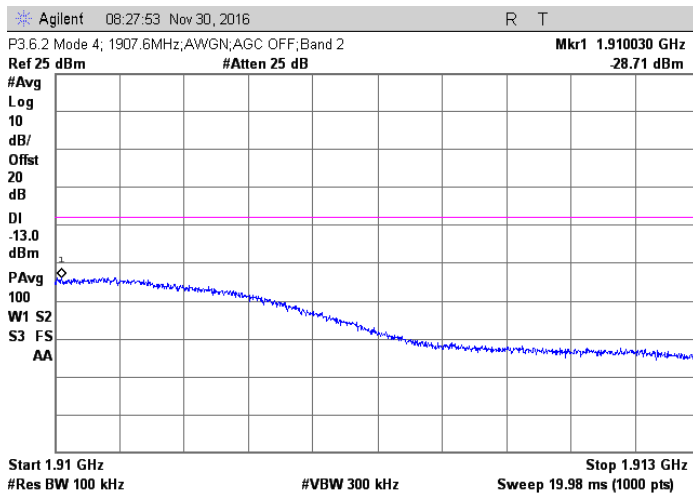
AWGN; 1907.6 MHz Injected Signal; AGC off
