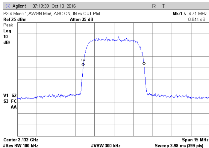
Amp output with AGC; 2.132 GHz; AWGN
