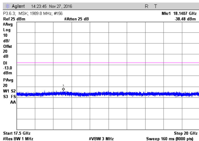
MSK; 1989.8 MHz Injected Signal
