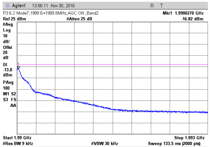
MSK; 1989.6 + 1989.8 MHz Injected Signals; AGC on
