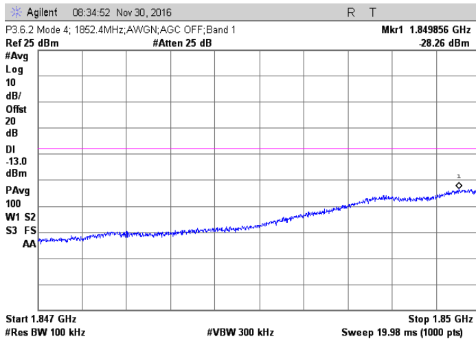
AWGN; 1852.4 MHz Injected Signal; AGC off
