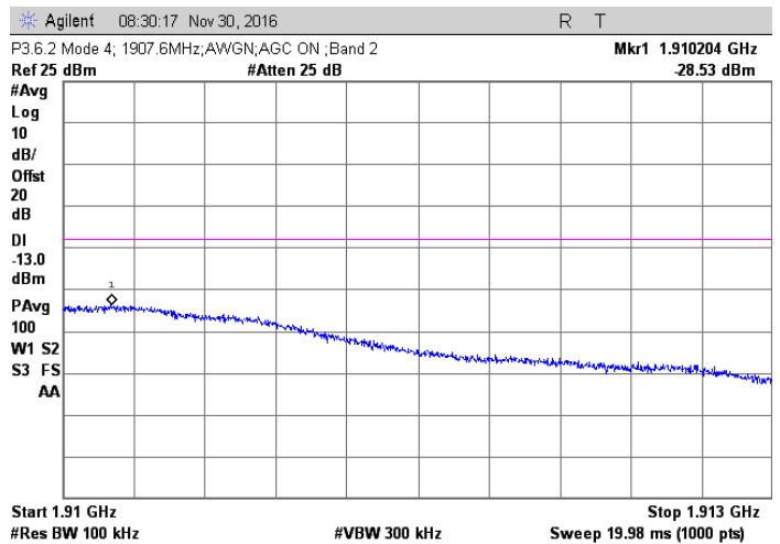
AWGN; 1907.6 MHz Injected Signal; AGC on
