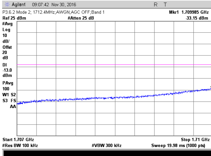
AWGN; 1712.4 MHz Injected Signal; AGC off
