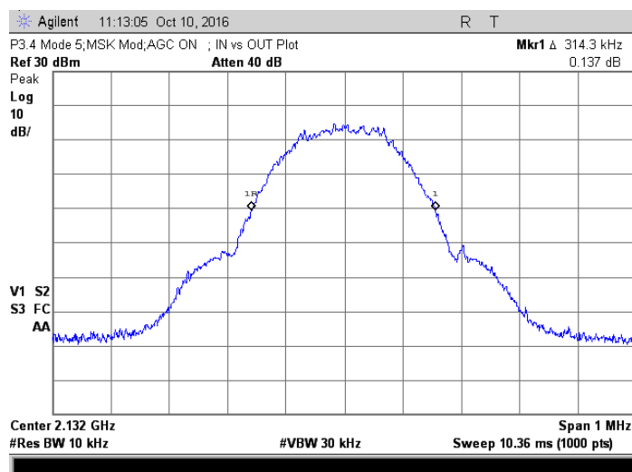
Amp output with AGC; 2.132 GHz, MSK
