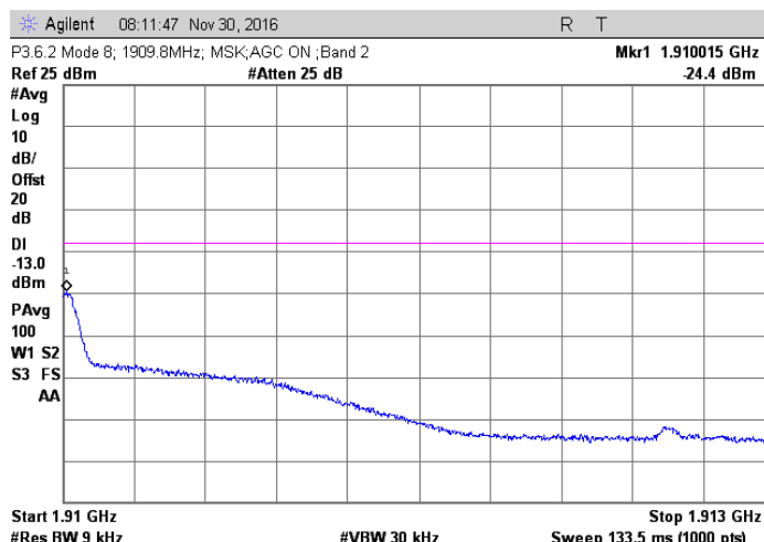
MSK; 1909.8 MHz Injected Signal; AGC on
