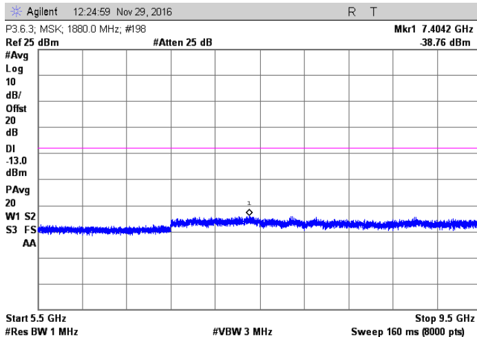
MSK; 1880 MHz Injected Signal
