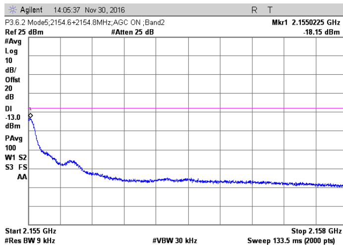
MSK; 2154.6 + 2154.8 MHz Injected Signals; AGC on
