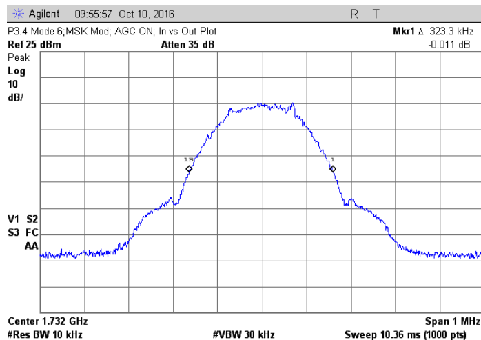
Amp output with AGC; 1.732 GHz, MSK
