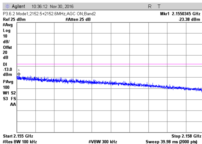
AWGN; 2152.5 + 2152.6 MHz Injected Signals; AGC on
