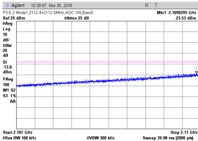
AWGN; 2112.4 + 2112.5 MHz Injected Signals; AGC on
