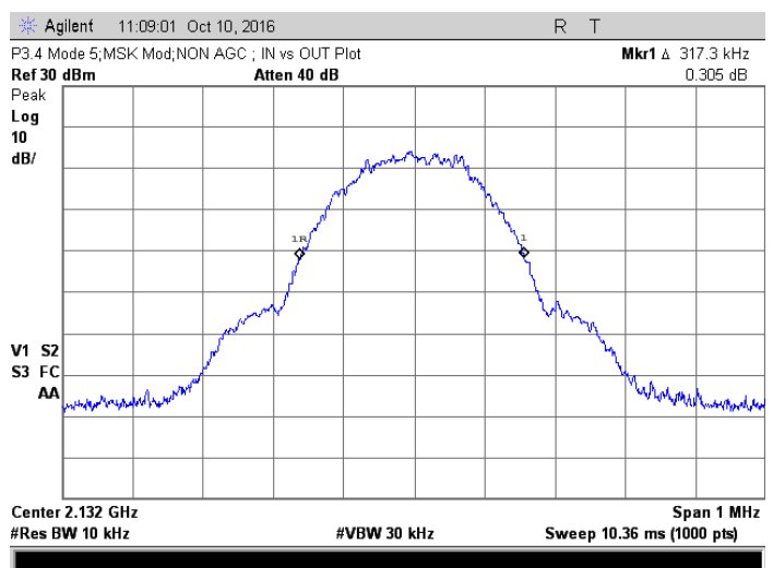
Amp output, no AGC; 2.132 GHz, MSK
