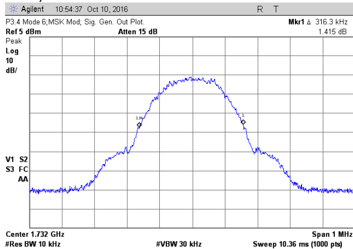
Generator output; 1.732 GHz, MSK
