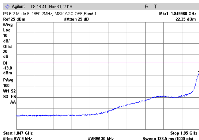
MSK; 1850.2 MHz Injected Signal; AGC off
