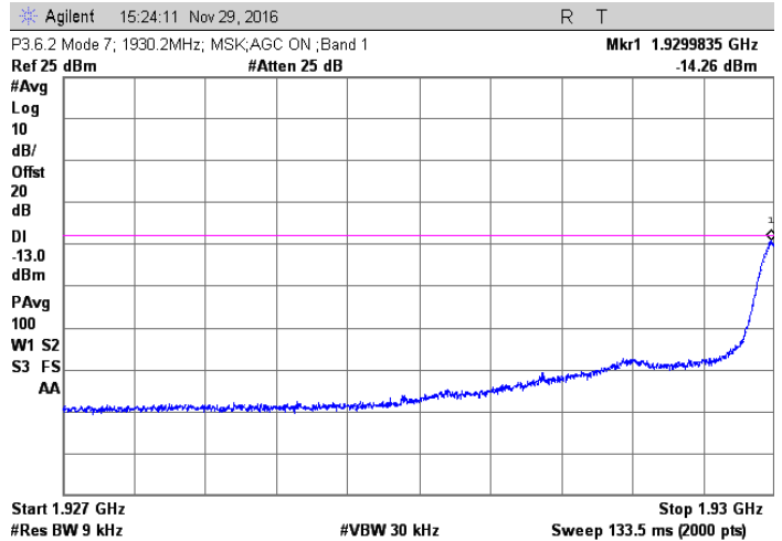
MSK; 1930.2 MHz Injected Signal; AGC on
