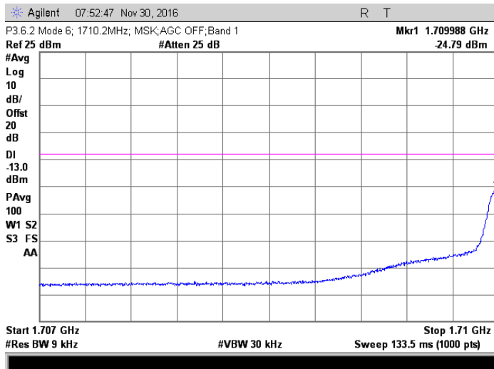
MSK; 1710.2 MHz Injected Signal; AGC off
