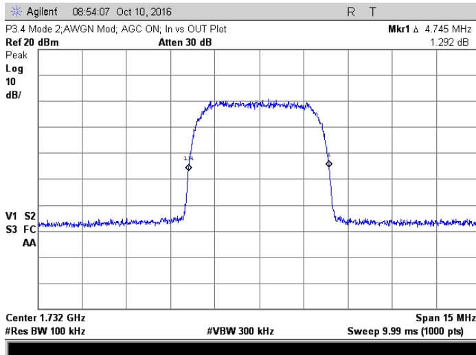
Amp output with AGC; 1.732 GHz, AWGN
