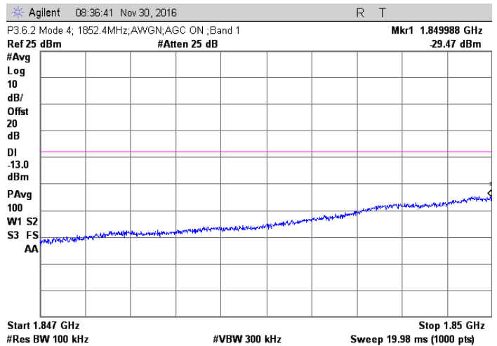
AWGN; 1852.4 MHz Injected Signal; AGC on
