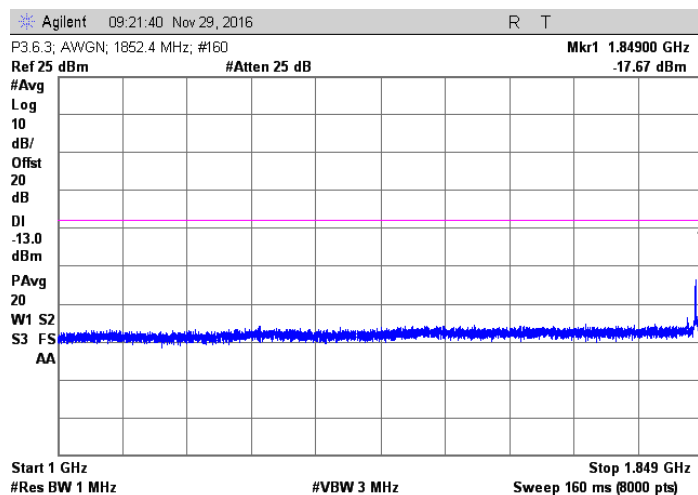
AWGN; 1852.4 MHz Injected Signal
