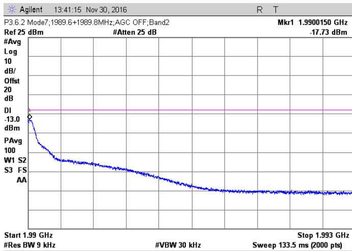
MSK; 1989.6 + 1989.8 MHz Injected Signals; AGC off
