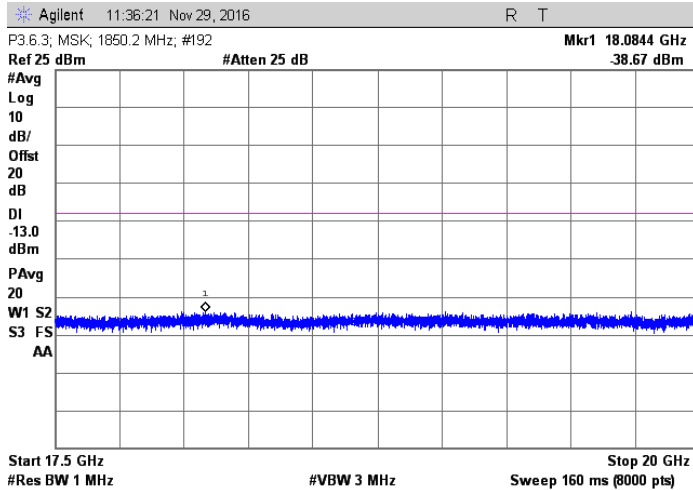
MSK; 1850.2 MHz Injected Signal
