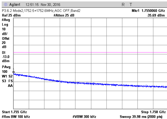
AWGN; 1752.5 + 1752.6 MHz Injected Signals; AGC off
