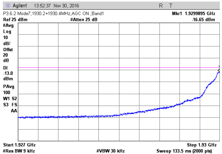
MSK; 1930.2 + 1930.4 MHz Injected Signals; AGC on
