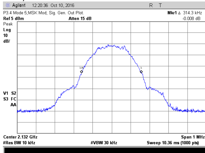
Generator output; MSK 2.132 GHz, MSK
