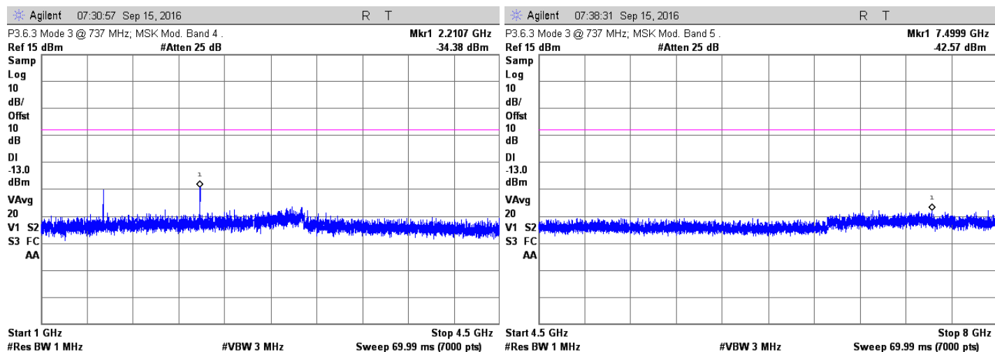
MSK; 737 MHz Injected Signal
