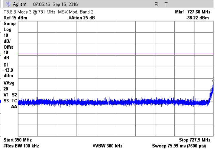
MSK; 731 MHz Injected Signal
