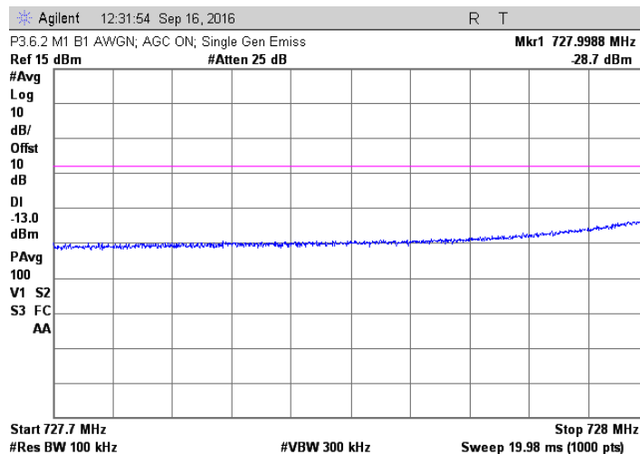
AWGN; 730.5 MHz Injected Signal; AGC on
