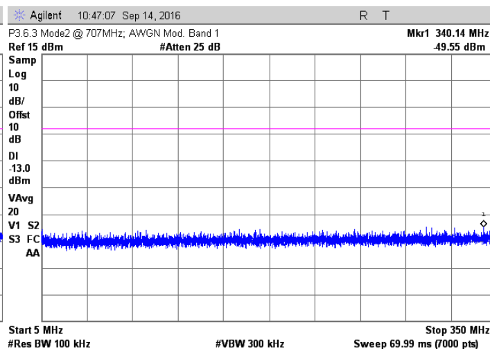
AWGN; 707 MHz Injected Signal
