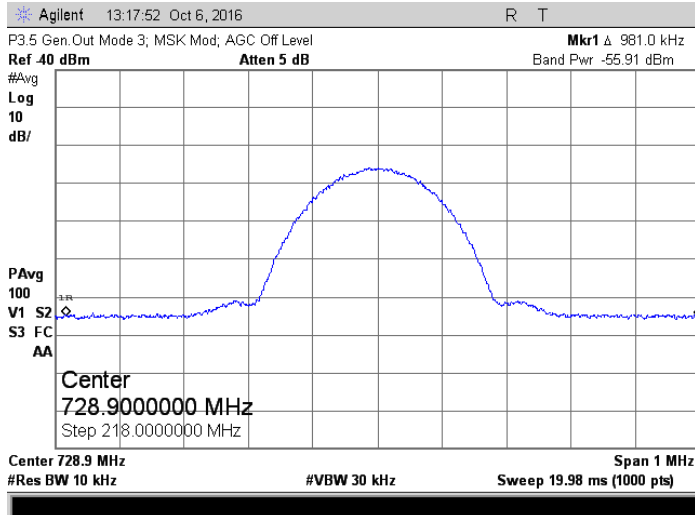
728.9 MHz MSK; Generator Out
