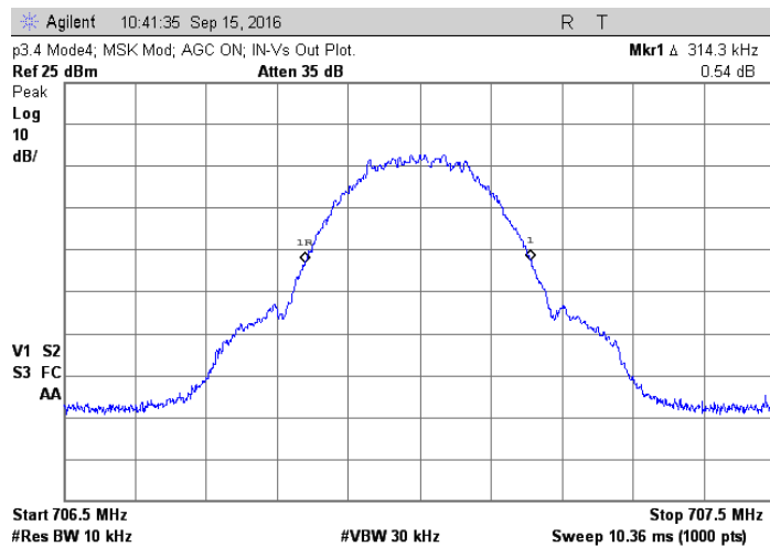
Amp output with AGC; 707 MHz, MSK
