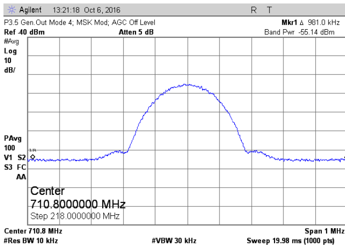
710.8 MHz MSK; Generator Out
