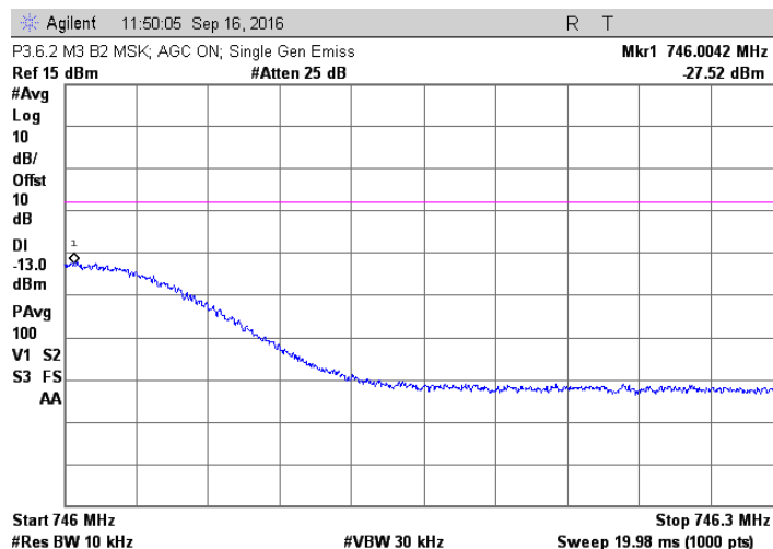
MSK; 745.8 MHz Injected Signal; AGC on
