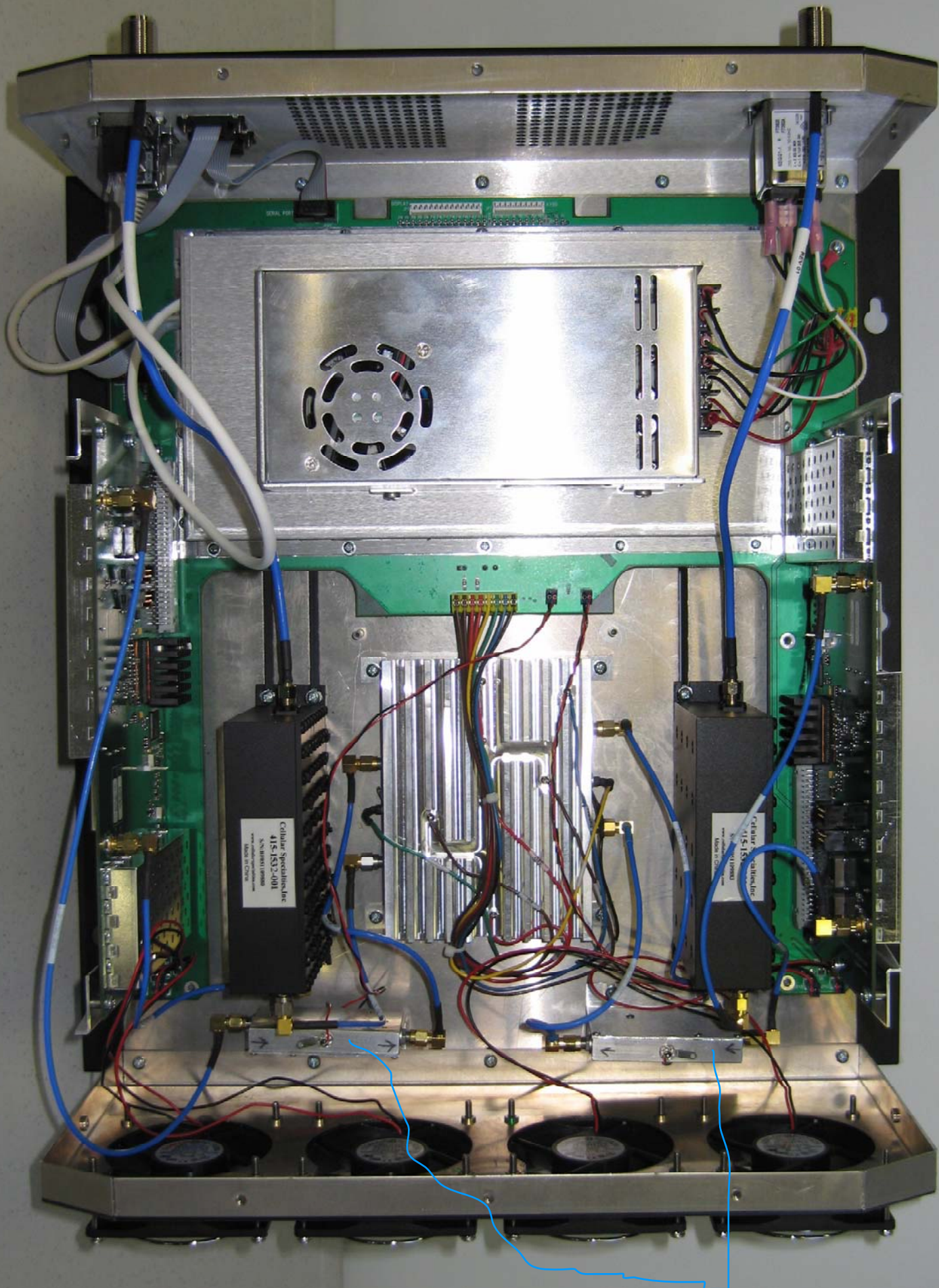
PRE-AMPLIFIERS
