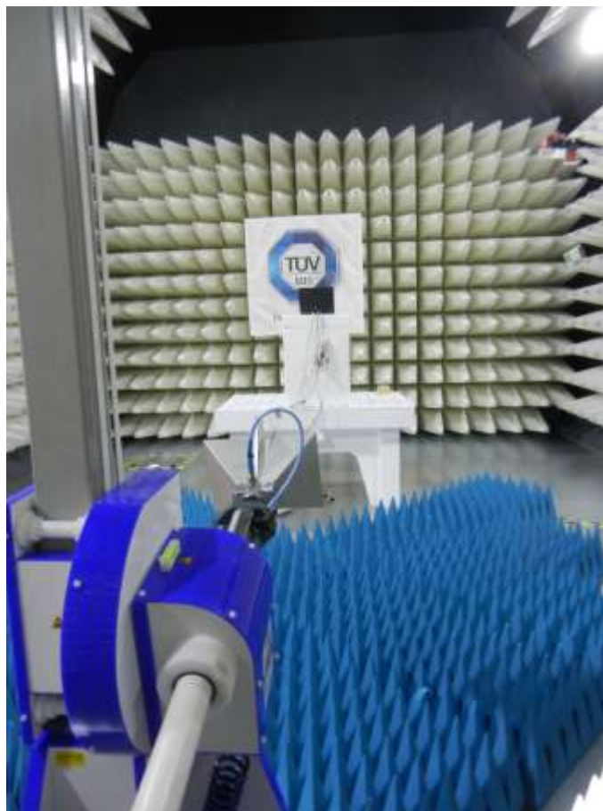
Figure 4: Radiated Emissions above 1 Gz
