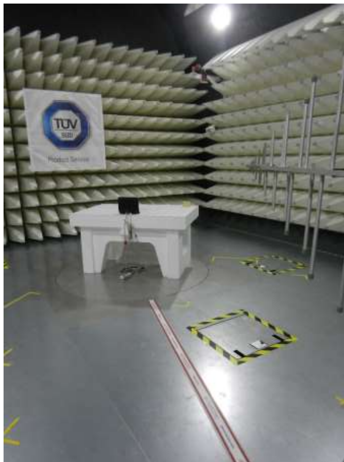
Figure 3 Radiated Emissions 30 MHz -w 1 GHz
