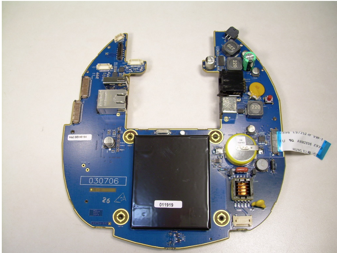
Side A of the Main PCB
