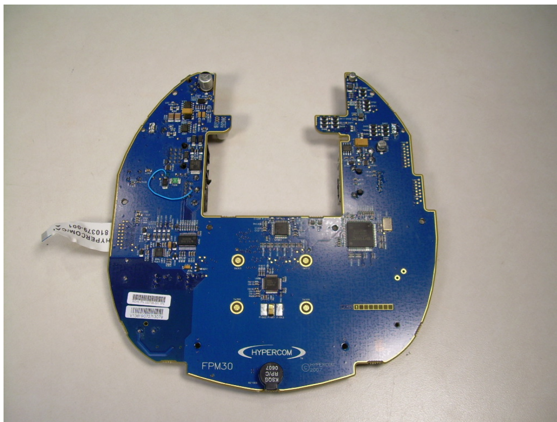
Side B of the Main PCB
