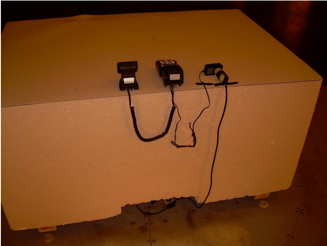
Back View Radiated Disturbance Stand Alone Configuration
