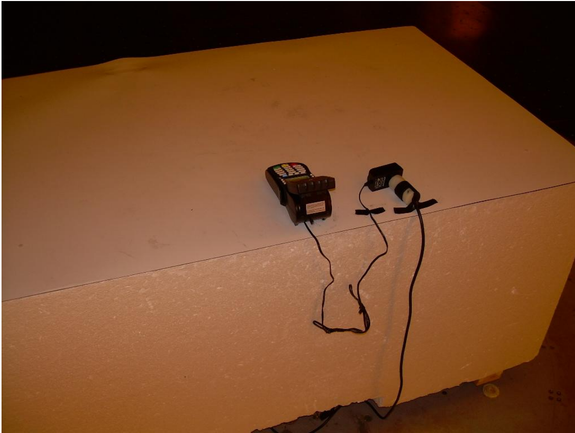
Back View Radiated Disturbance Clip On Configuration
