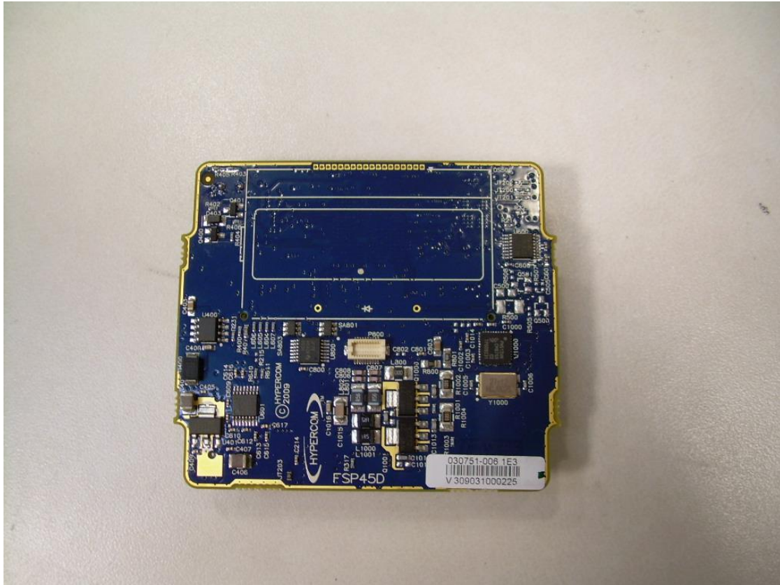
Front Side of the Main PCB
