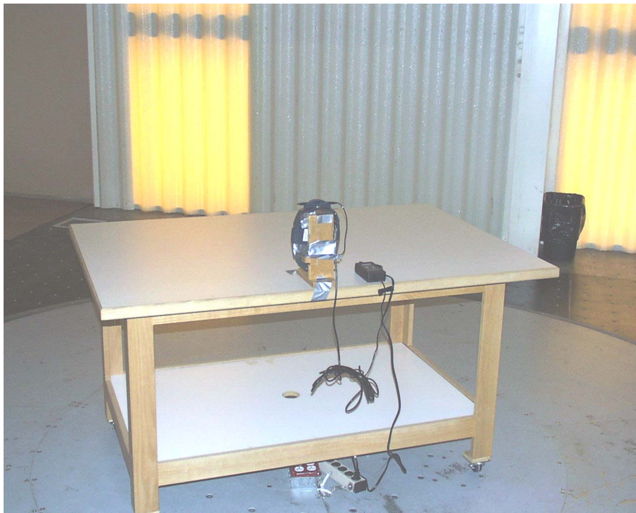
Photograph 2 - Back View of the Radiated Test Setup (Vertical Alignment)
