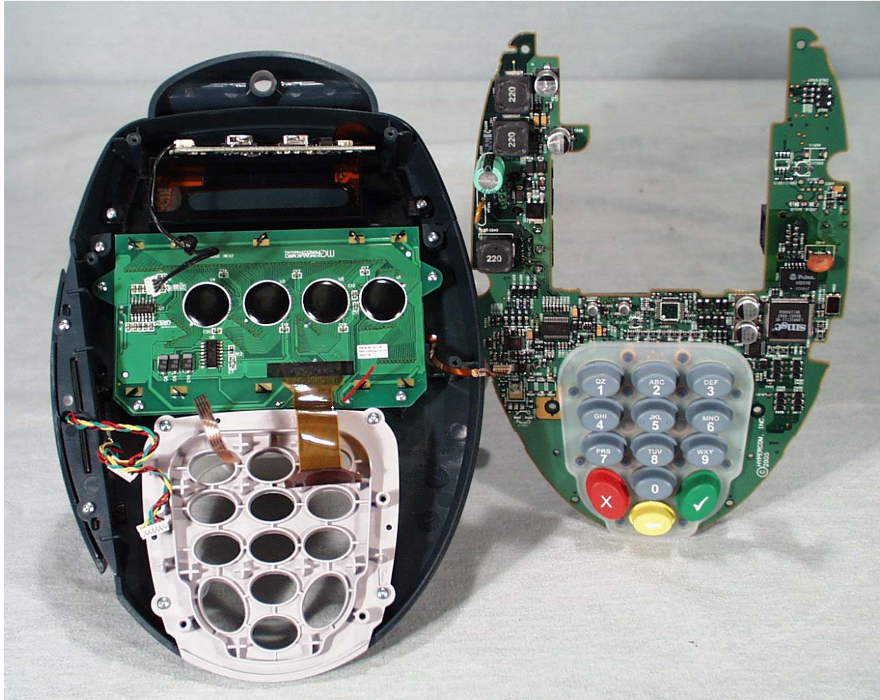
Photograph 10 - Internal View of the EUT
