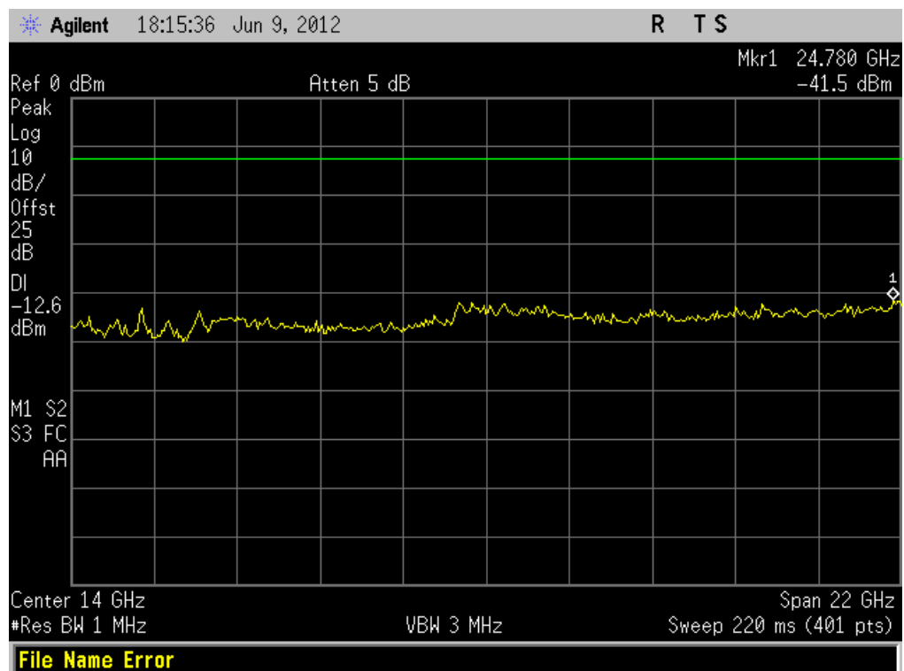
(Plot H.2: Channel = 39, 3GHz to 25GHz @ 8-DPSK)
