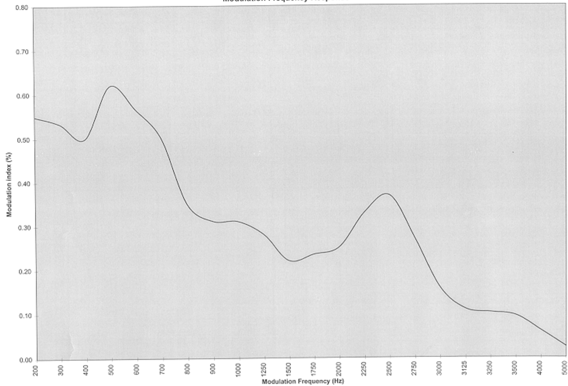
Modulation Frequency Response
