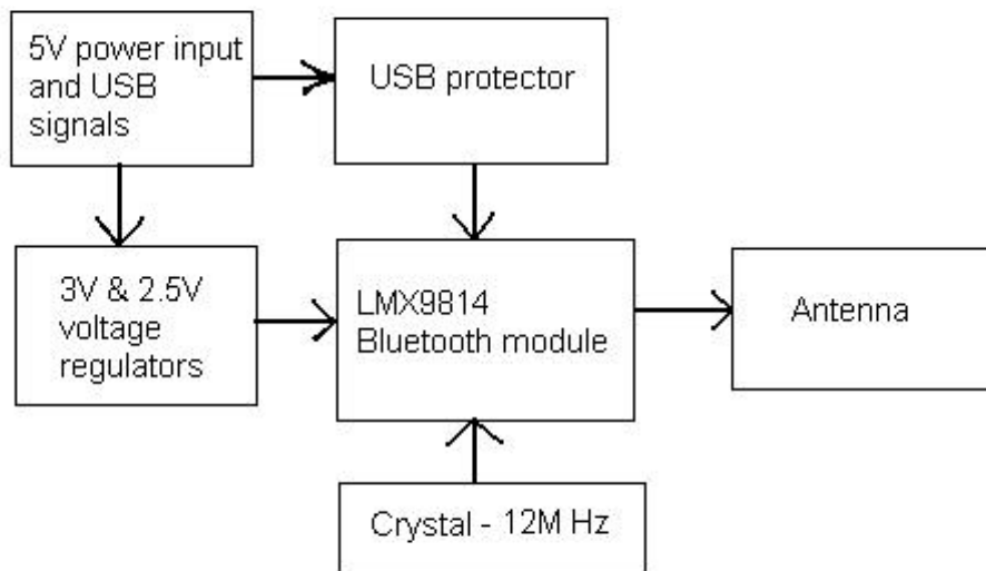
Abe Bluetooth USB Dongle - Block Diagram
