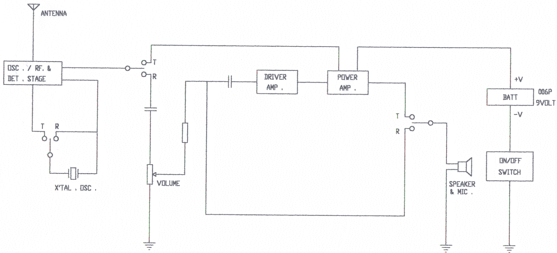
BLOCK DIAGRAM
