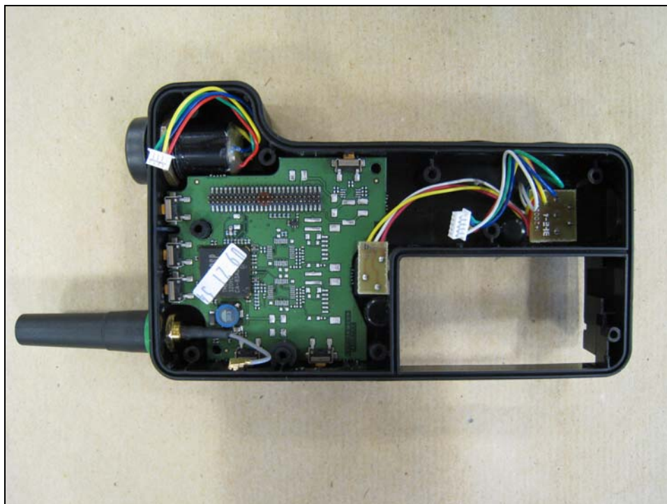
DC2912 – Lower pcb top
