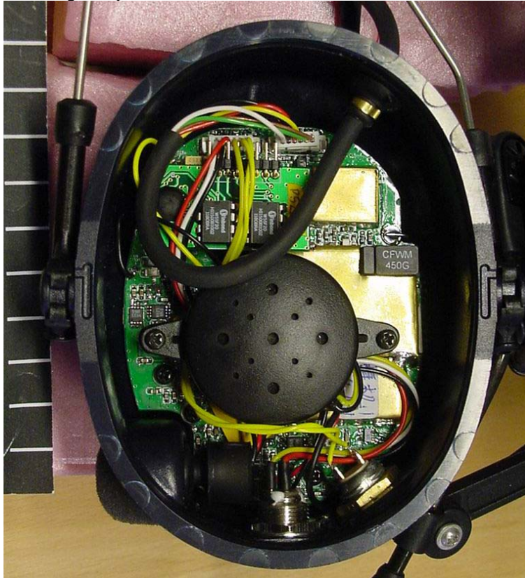
EUT, right cap inside, close-up (speaker dismounted)
