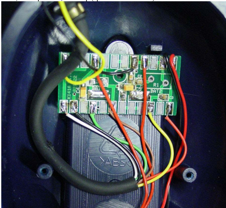
EUT, left cap inside, close-up (speaker dismounted)
