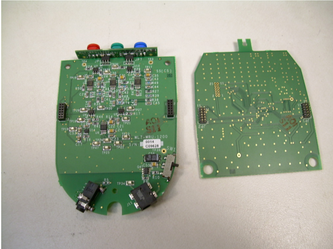
View of the EUT Boards Side A
