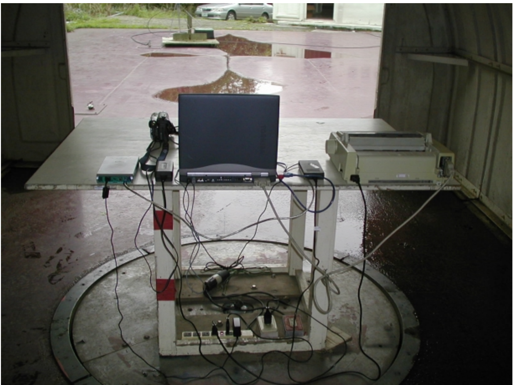
Set-up Photo ( Radiation Back )
