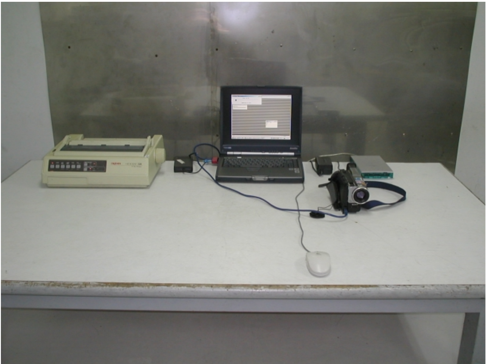
Set-up Photo ( Conduction Front )
