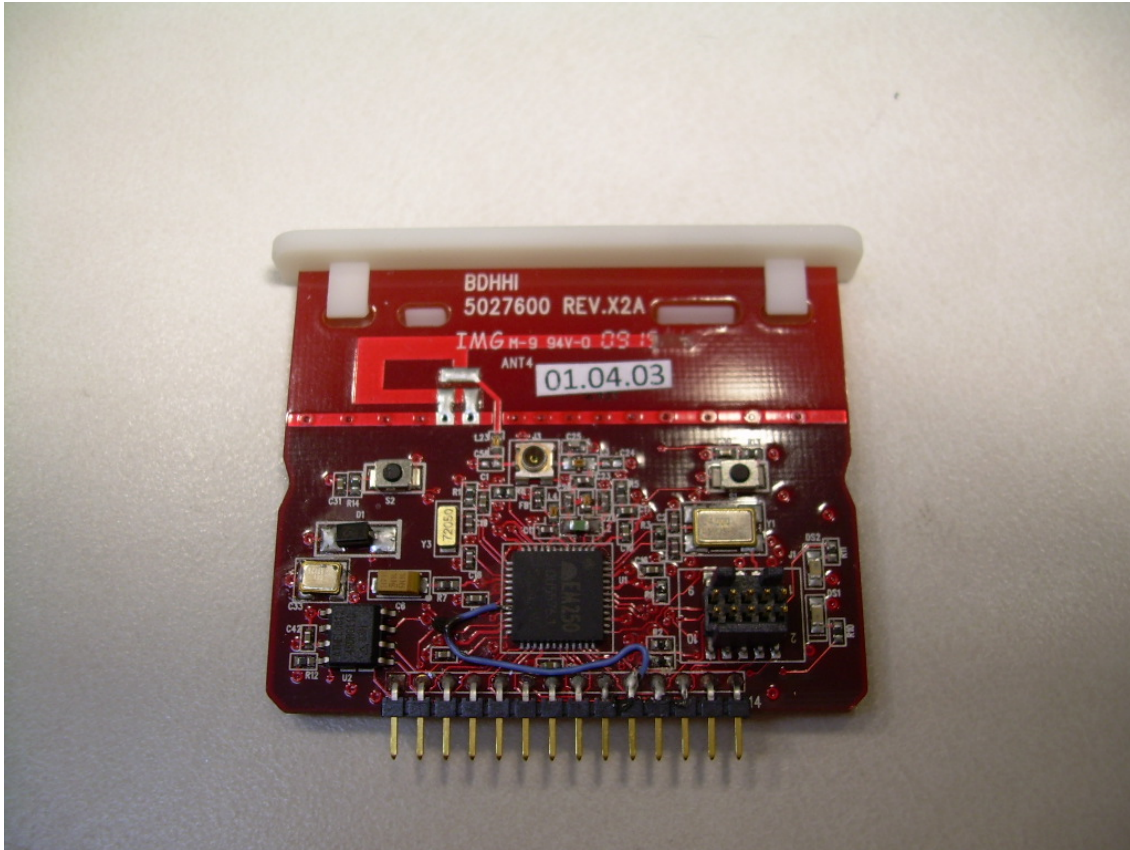
Photograph 7 - Side A of the Transceiver PCB
