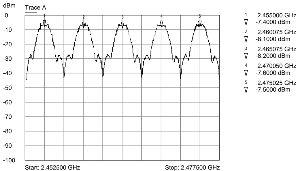
Trace A Upper 5 channels
