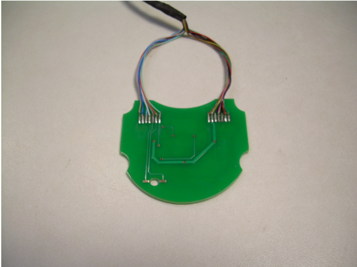
Photograph 10 - Side B of the Keypad PCB
