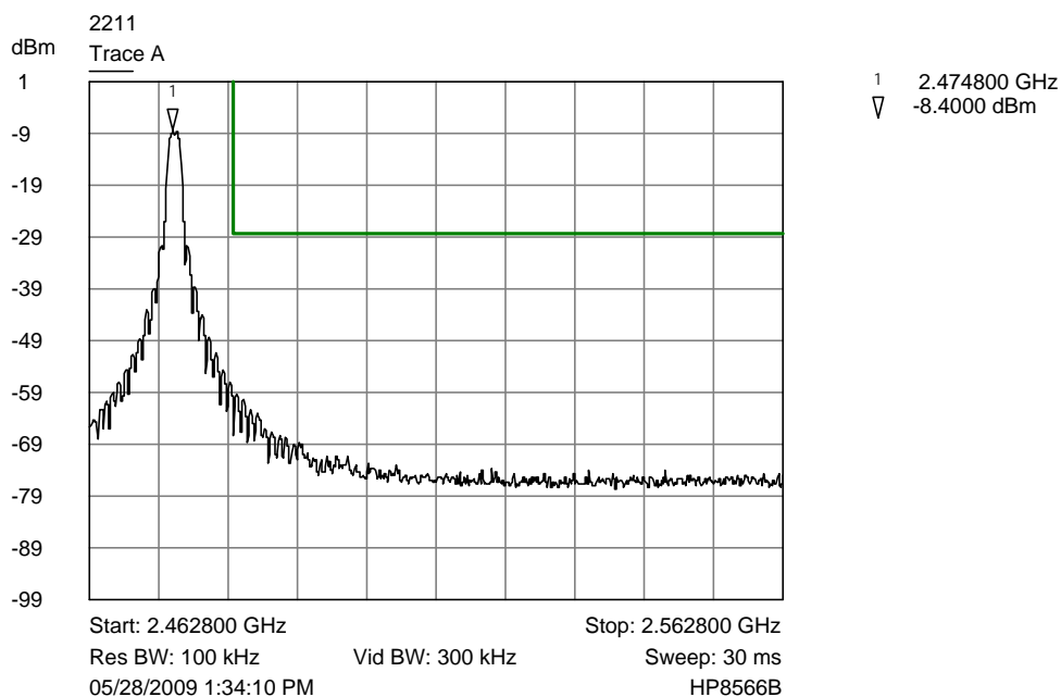
Trace A Upper channel band edge plot
