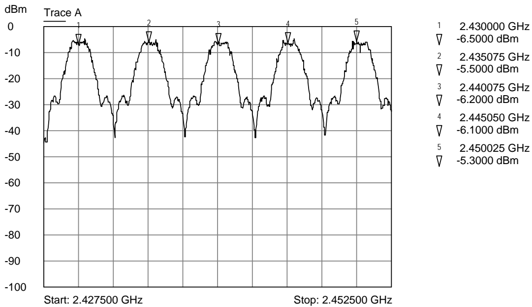
Trace A Middle 5 channels
