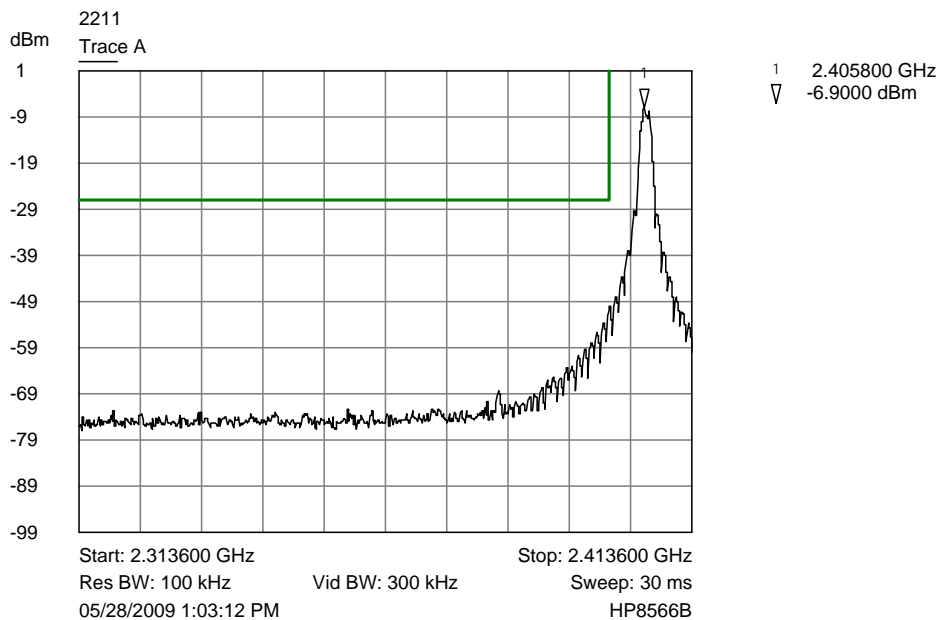
Trace A Lower channel band edge plot
