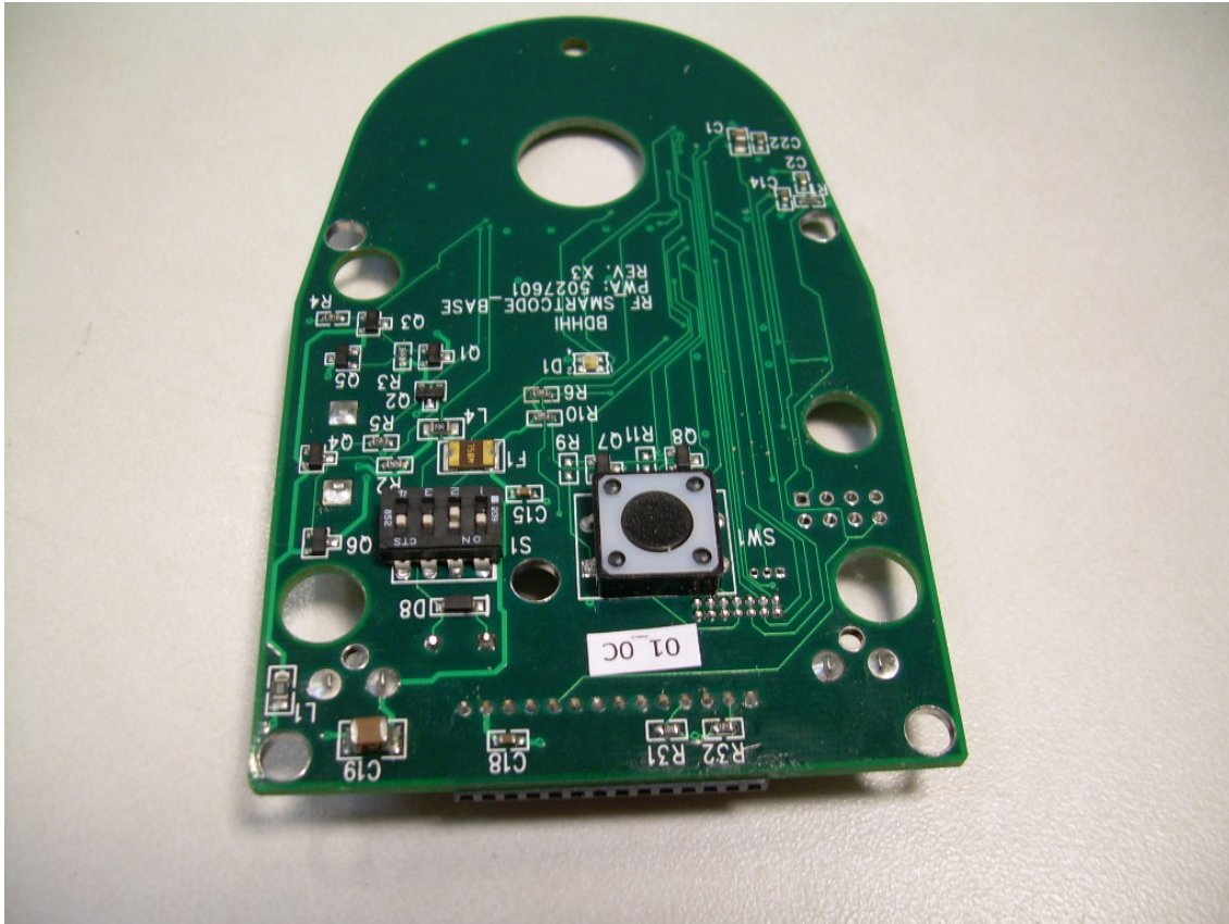
Photograph 5 - Side A of the Main PCB
