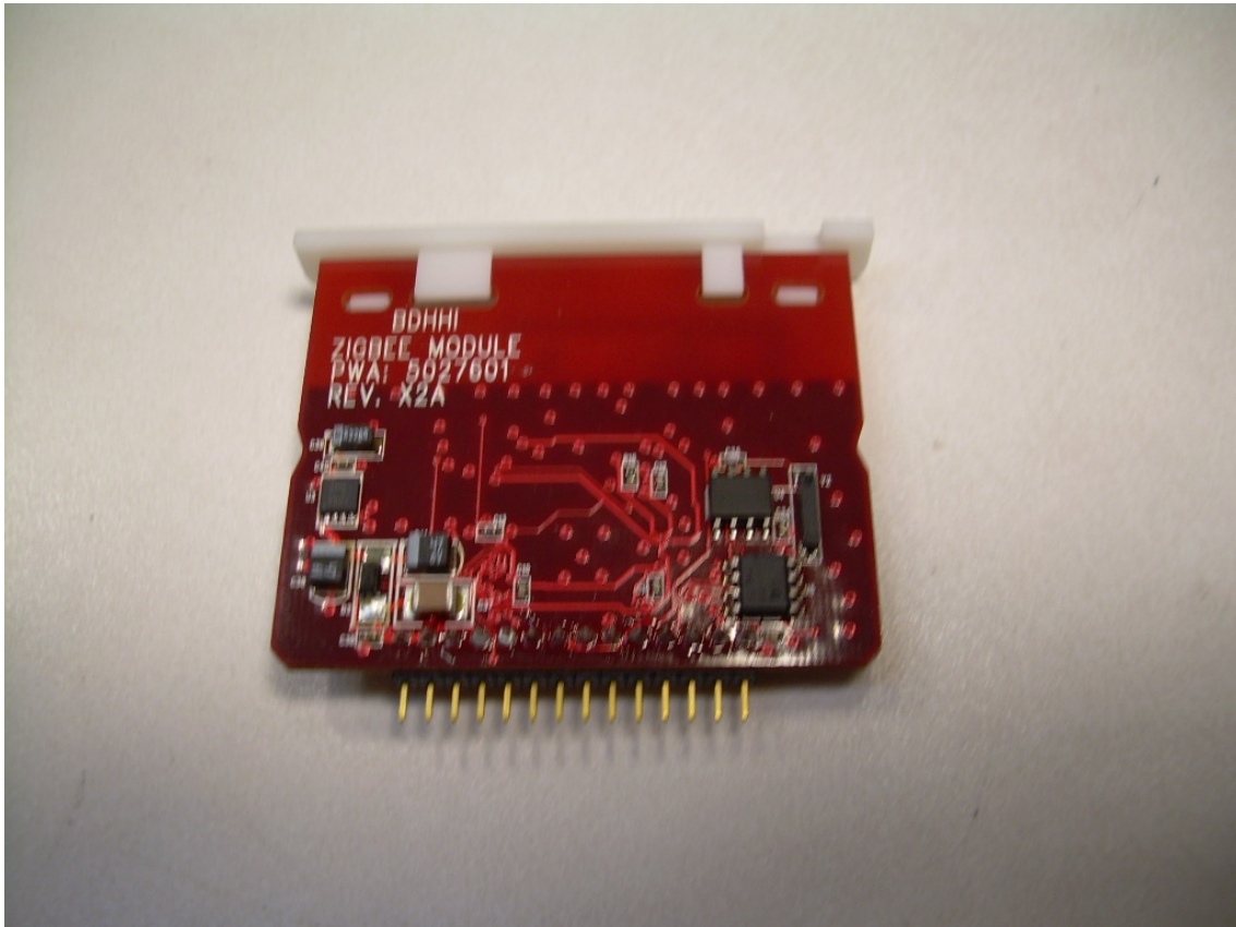
Side B of the Transceiver PCB
