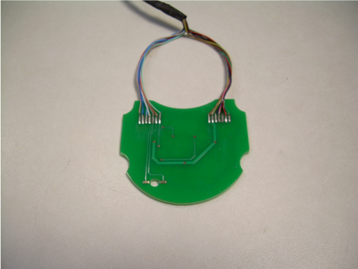
Side B of the Keypad PCB
