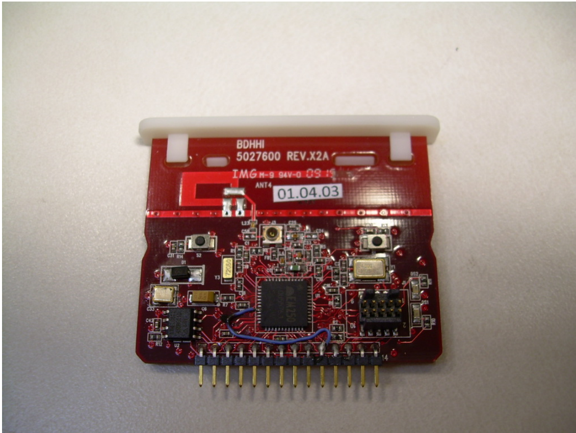
Side A of the Transceiver PCB
