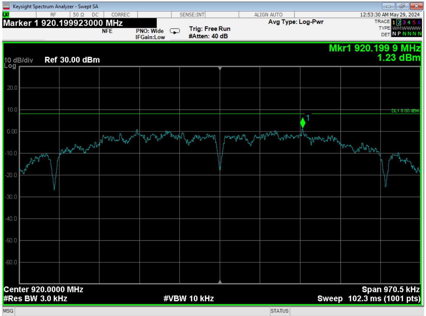
Spectral Density Output – High Channel
