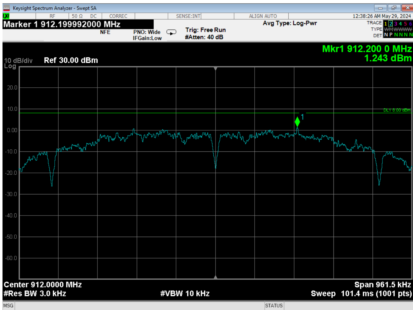
Spectral Density Output – Low Channel
