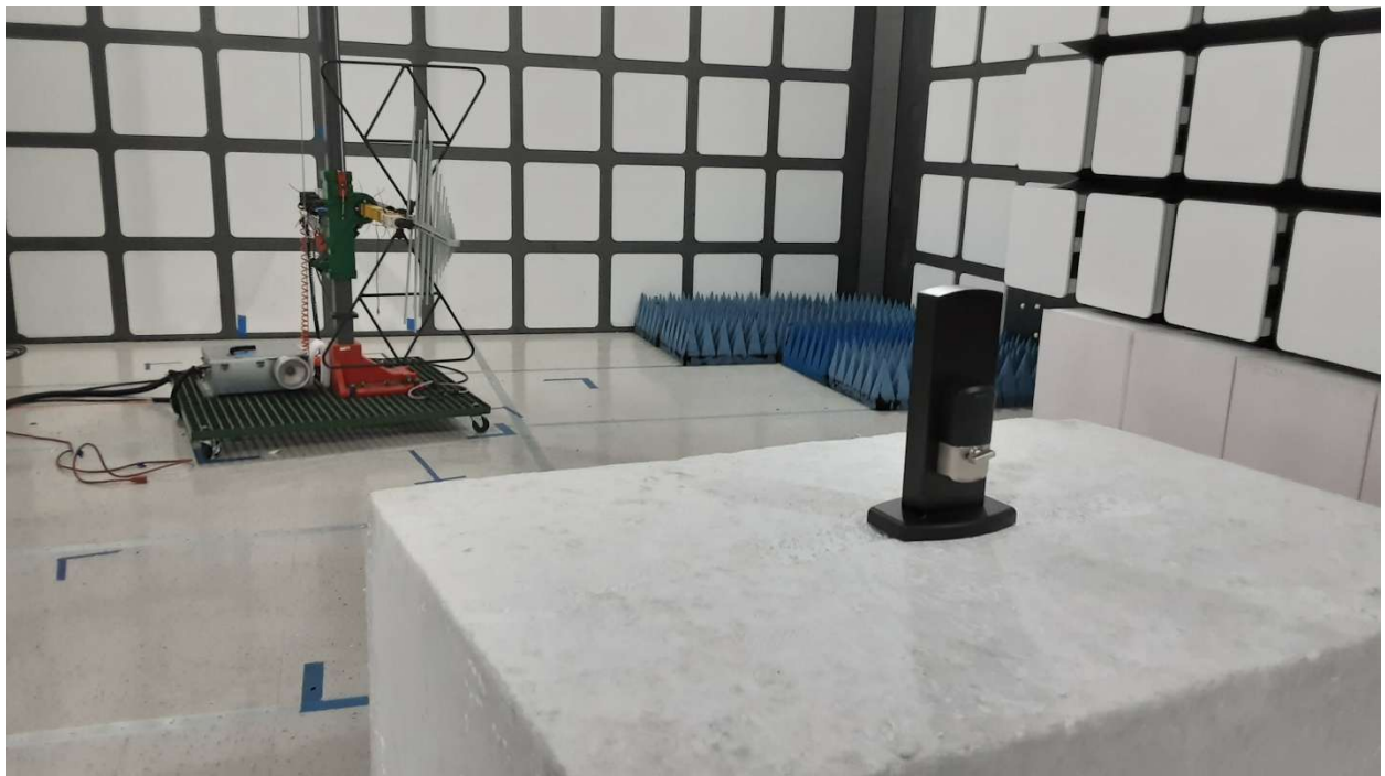
30 to 1GHz Emissions Set-Up
