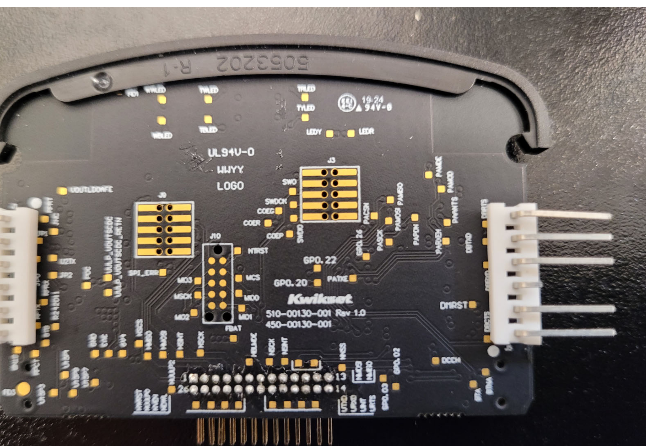
Bottom View of the RF Module with Label Removed - View 1
