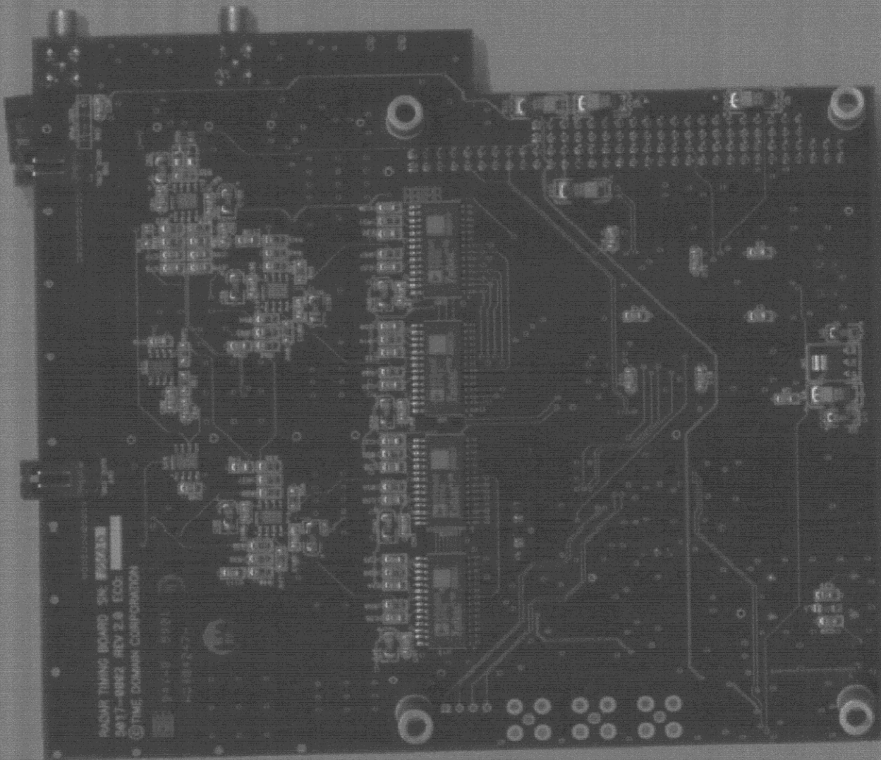
Timer Board-Bottom
