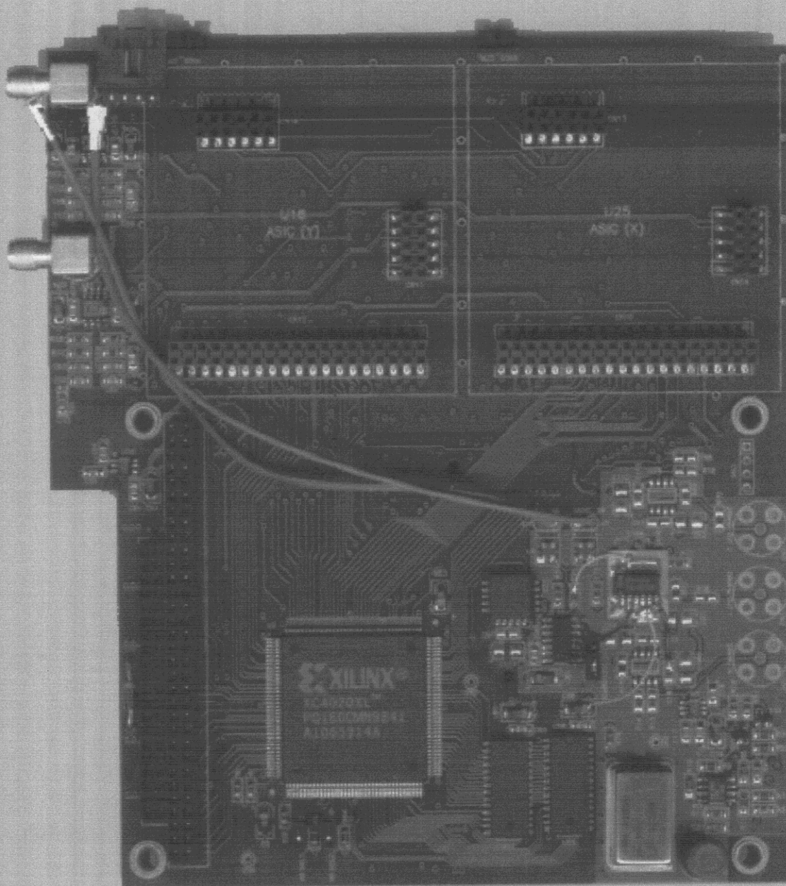
Timer Board-Top Without Panel
