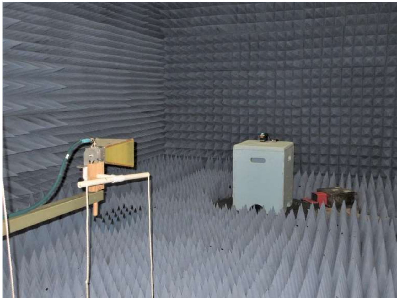
Radiated Above 1 GHz - USB Battery Bank Powered
