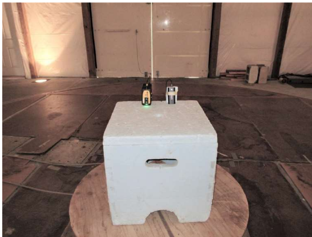
Radiated Below 1 GHz - USB Battery Bank Powered - Front
