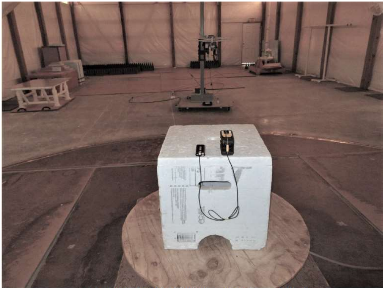
Radiated Below 1 GHz - USB Battery Bank Powered - Back
