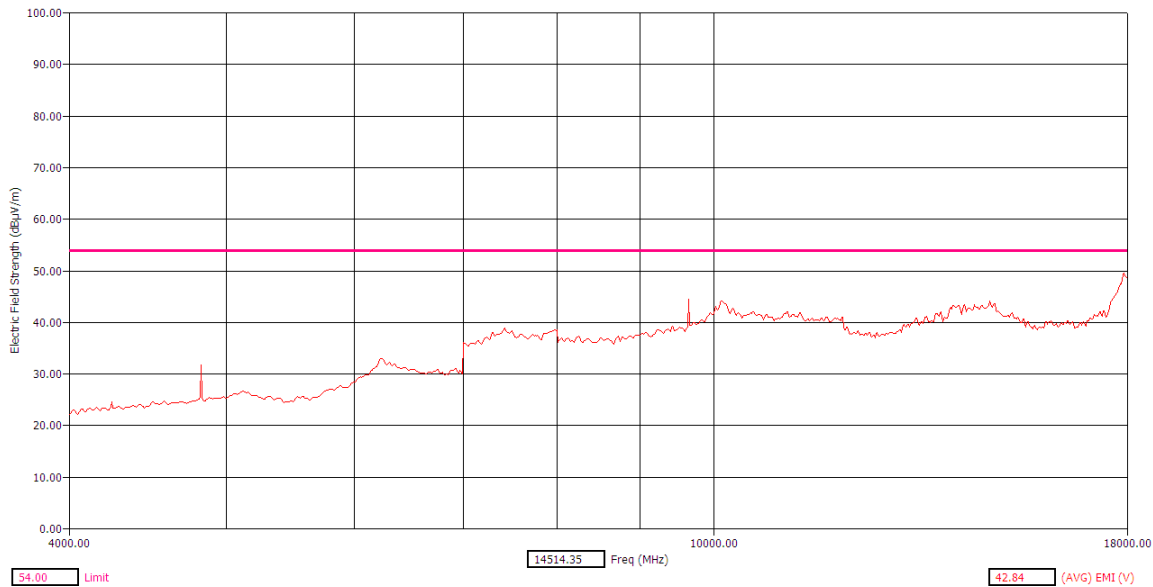
Figure 12: Radiated Emission (Average) – Vertical polarization – 4GHz to 18GHz – 802.11b, Channel 1
