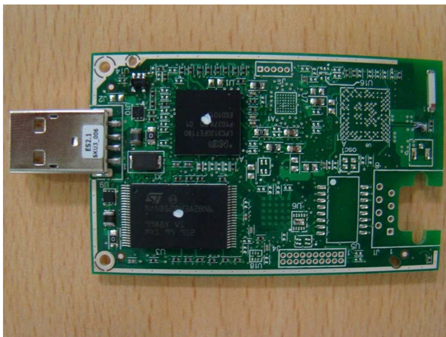
Figure 2: Internal view of the Product – Top side
