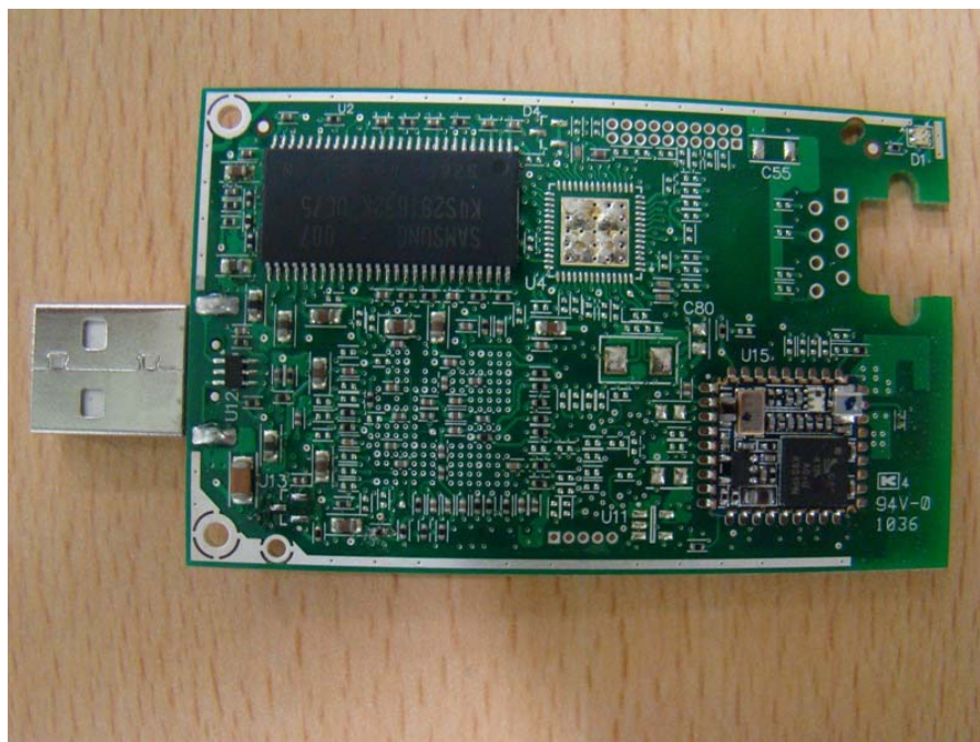
Figure 1: Internal view of the Product – Bottom side
