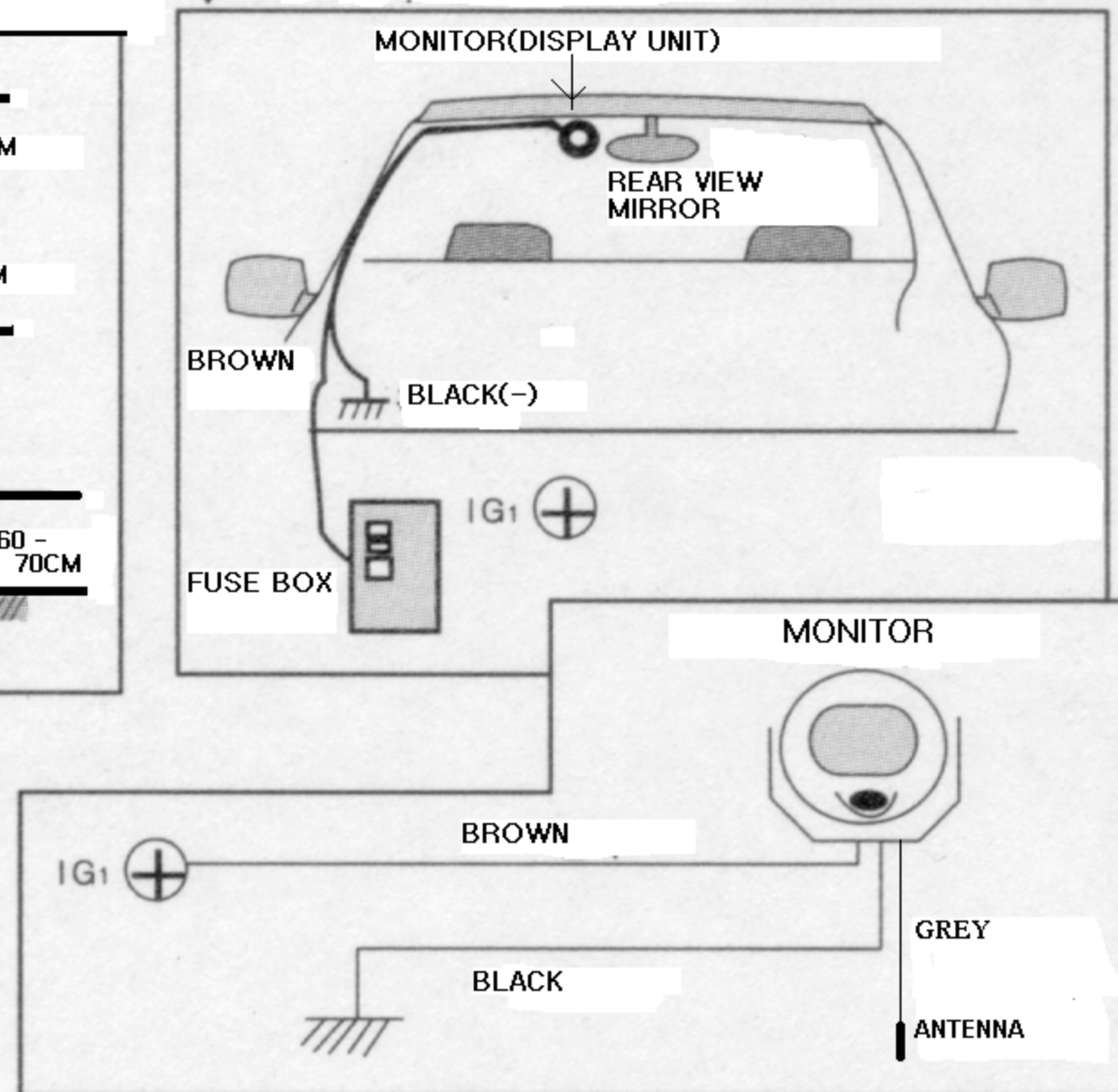
INSTALLATION & WIRING DIAGRAM CAR PARKING SENSOR MODEL : YPS-300M
