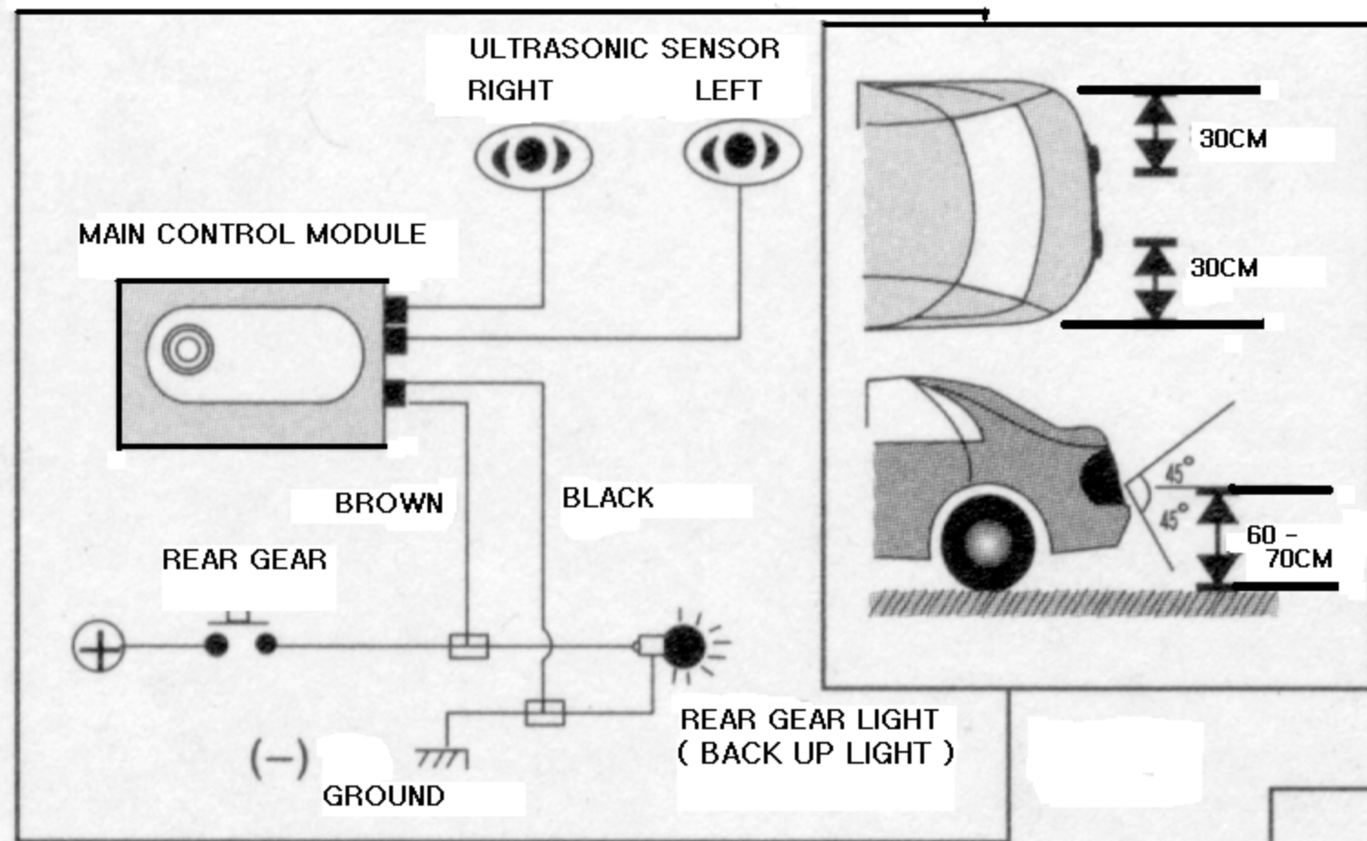
INSTALLATION & WIRING DIAGRAM CAR PARKING SENSOR MODEL : YPS-300M
