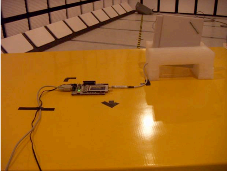
Radiated X-position, linear antenna
