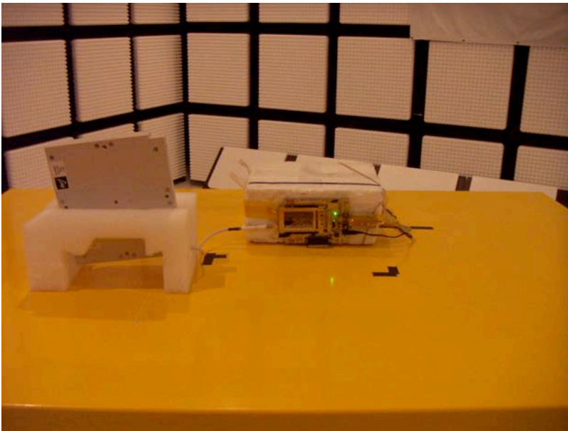
Y-position, linearly polarized antenna
