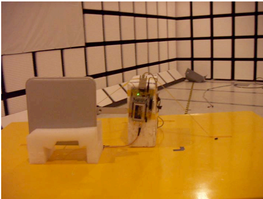
Z-position, circularly polarized antenna
