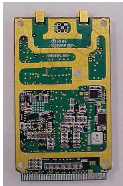
WJM3000 Bottom (unshielded)
