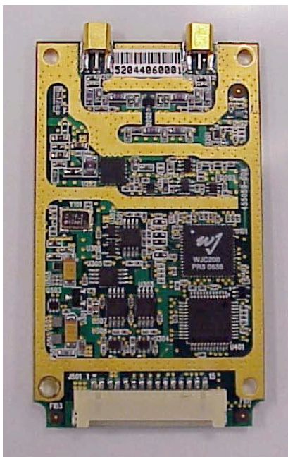
WJM3000 Top (unshielded)
