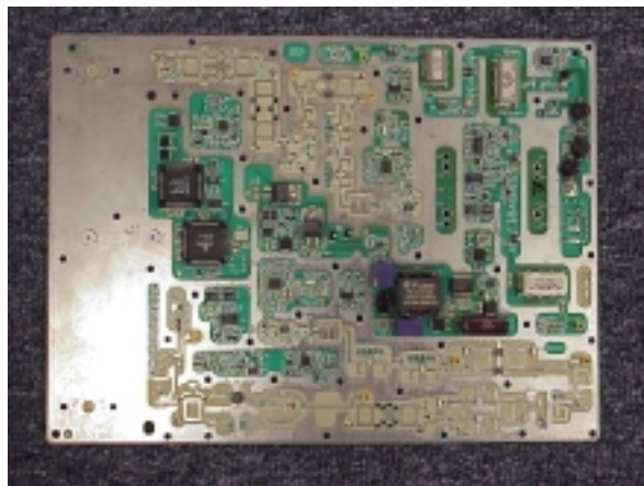
Board Front
