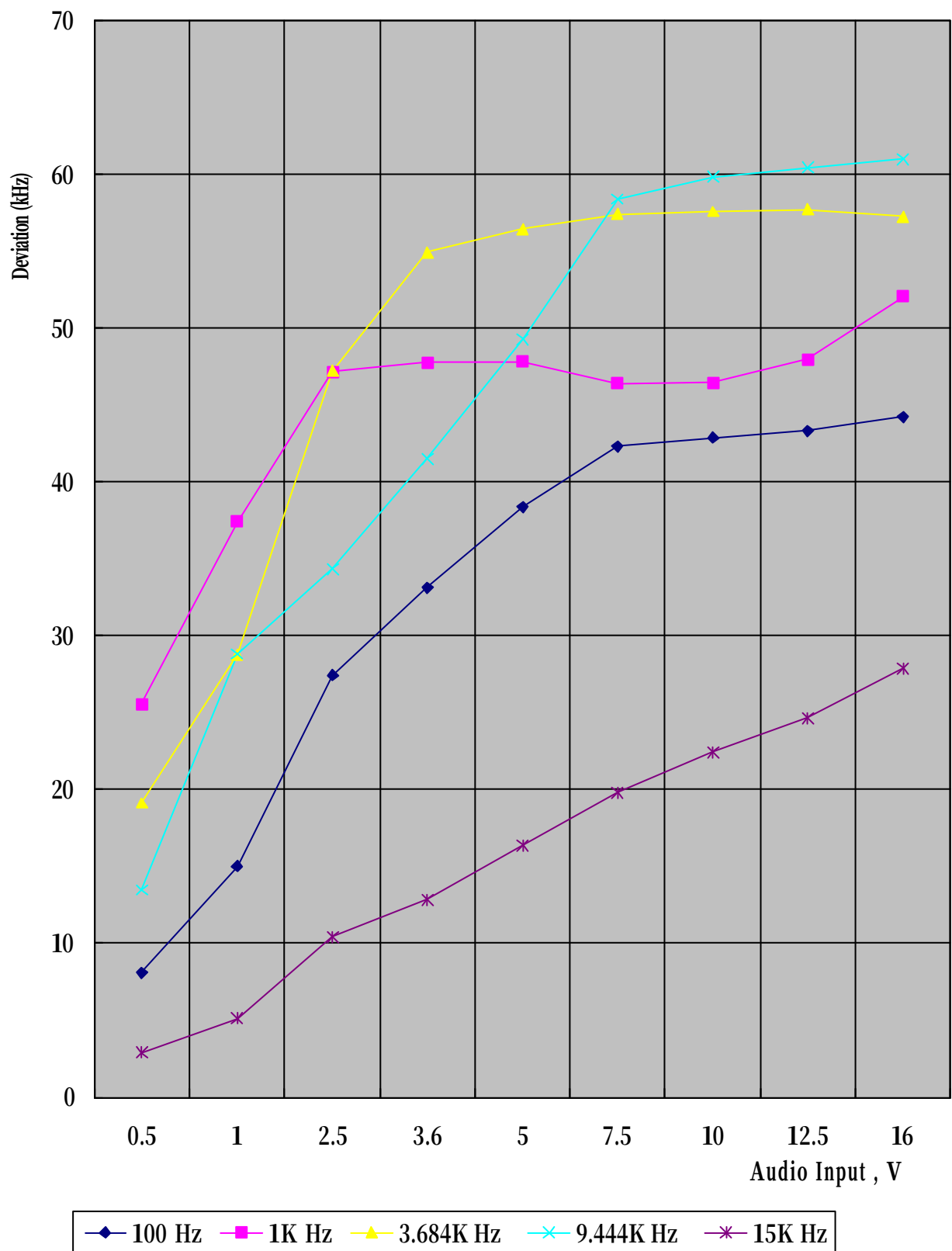
Chart 3.1 Modulation Limiting Measuerment Negative
