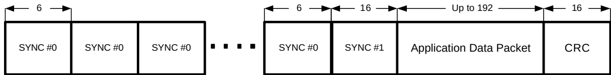
Figure 4: Wake Up Sequence and Receive Frame
