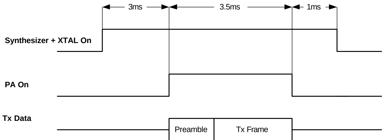
Figure 3: Transmit Timing
