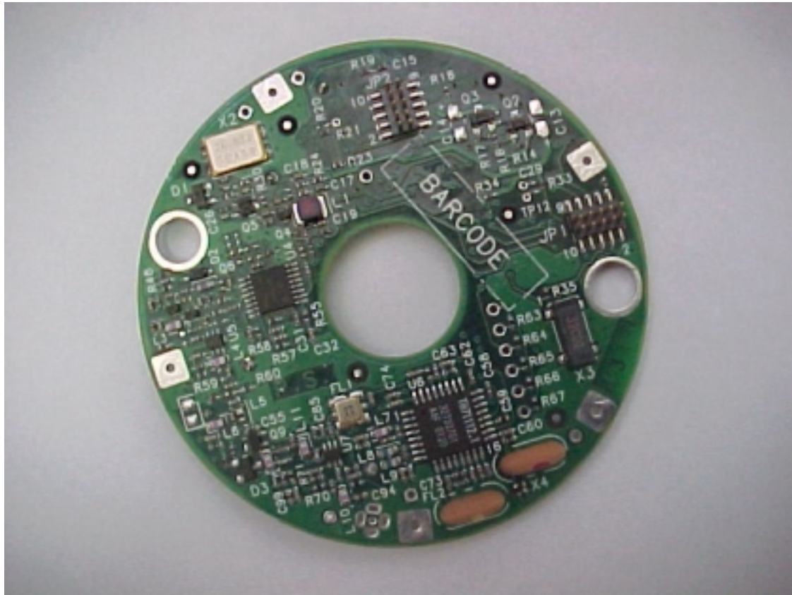
PCB first side
