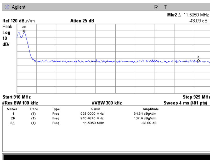
Plot 7.4.2 The highest high band edge emission, FSK modulation
