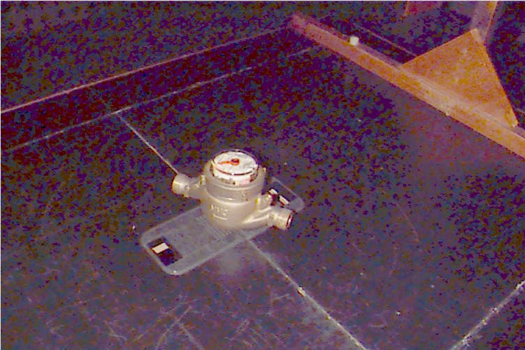
Radiated emission test setup, 2 – 9.3 GHz frequency range, close view
