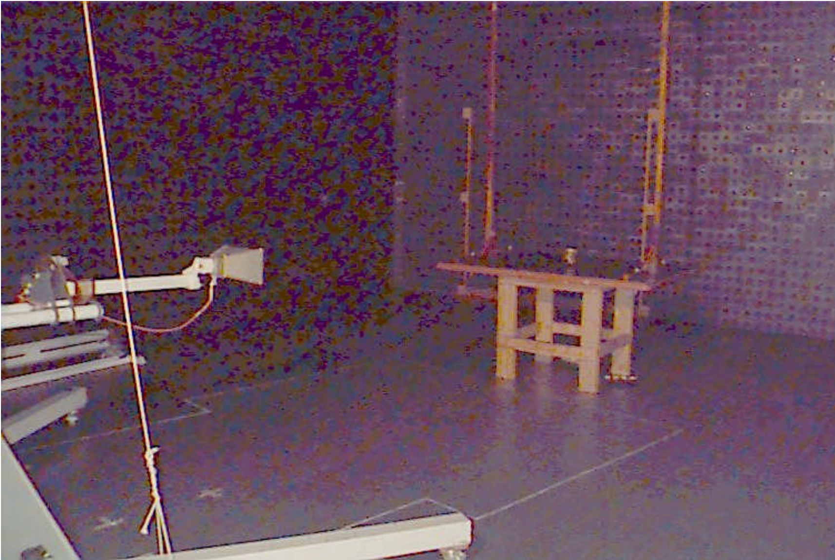
Radiated emission test setup, 2 – 9.3 GHz frequency range, general view
