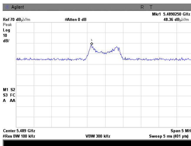
Plot 7.7.42 Radiated emission measurements at the sixth harmonic of high carrier frequency
