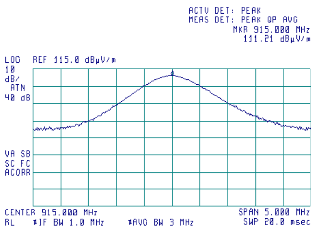
Plot 7.5.17 Field strength of carrier at mid frequency
