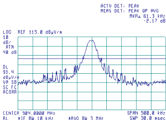
Plot 7.1.6 The 20 dB bandwidth test result at low frequency
