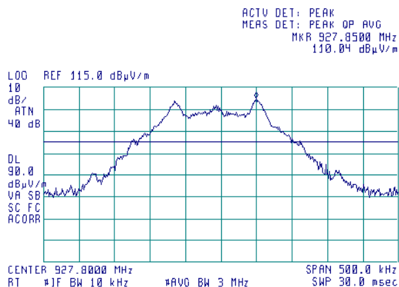
Plot 7.1.16 The 20 dB bandwidth test result at high frequency
