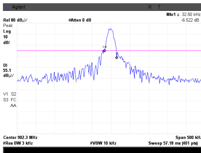
Plot 7.2.2 The 20 dB bandwidth test result at low frequency
