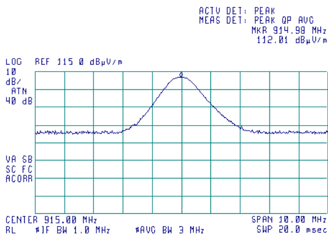
Plot 7.6.8 Field strength of carrier at mid frequency
