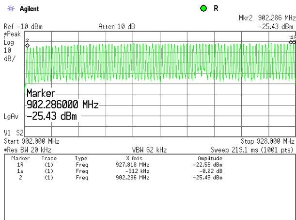
Plot 7.4.4 Number of hopping frequencies
