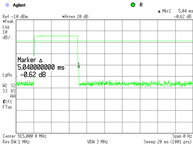
Plot 7.5.3 Single transmission duration
