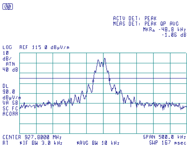
Plot 7.2.14 The 20 dB bandwidth test result at high frequency
