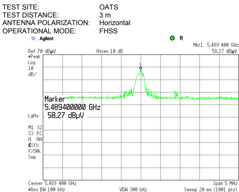
Plot 7.8.63 Radiated emission measurements at the sixth harmonic of mid carrier frequency
