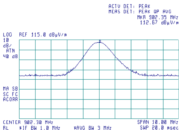
Plot 7.6.6 Field strength of carrier at mid frequency
