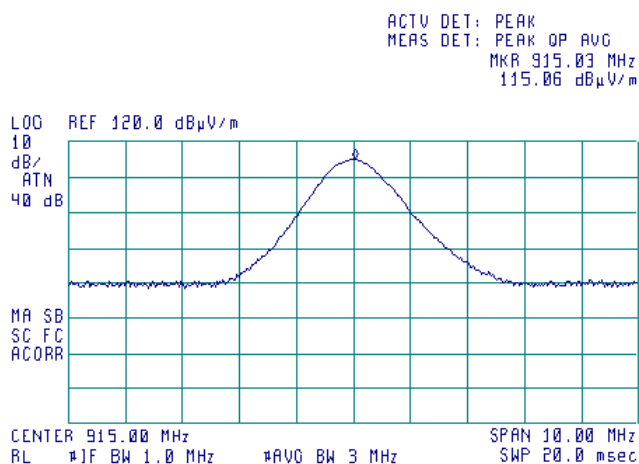
Plot 7.6.20 Field strength of carrier at mid frequency
