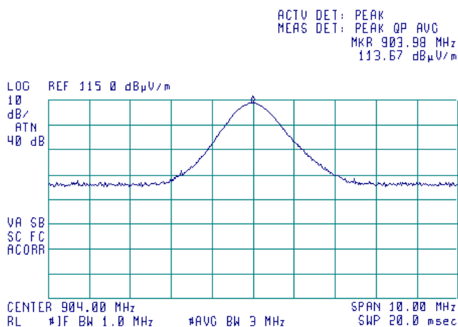
Plot 7.6.18 Field strength of carrier at low frequency
