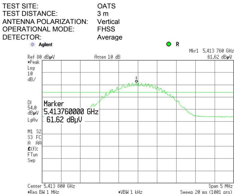
Plot 7.8.59 Radiated emission measurements at the sixth harmonic of low carrier frequency
