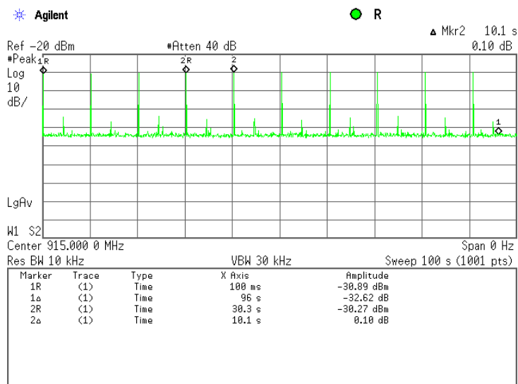
Plot 7.5.2 Single transmission period
