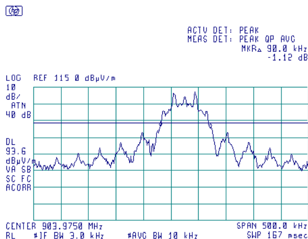
Plot 7.2.8 The 20 dB bandwidth test result at mid frequency
