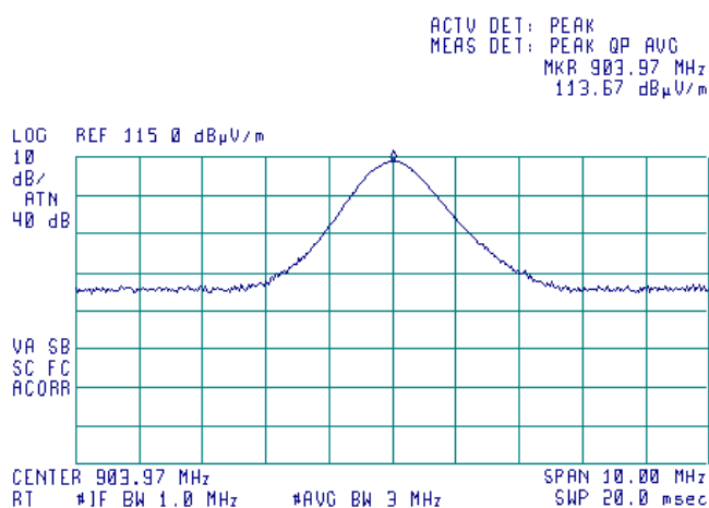
Plot 7.6.16 Field strength of carrier at low frequency
