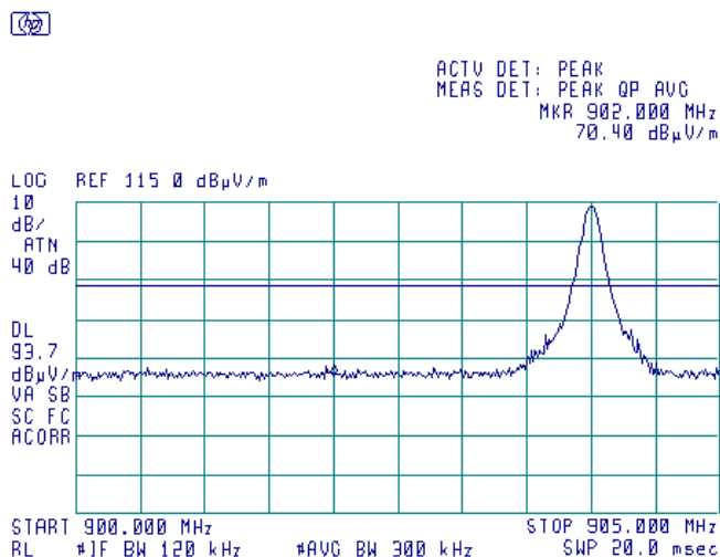
Plot 7.7.19 The highest band edge emission at low carrier frequency with hopping function disabled
