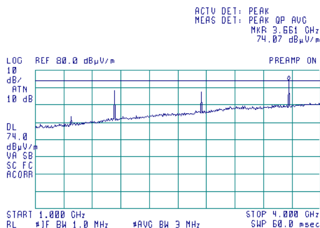
Plot 7.8.16 Radiated emission measurements from 1000 to 4000 MHz at the mid carrier frequency
