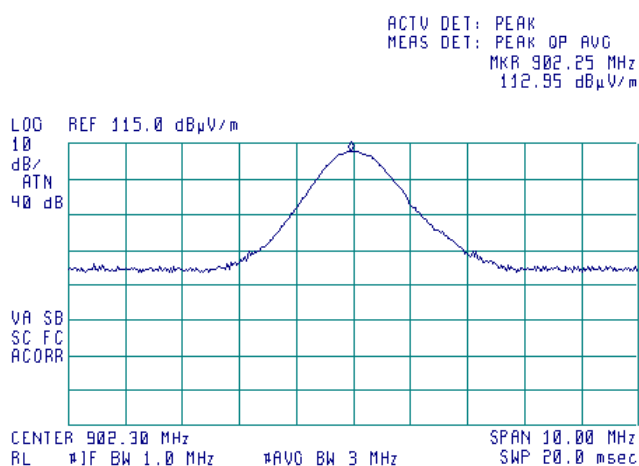
Plot 7.6.2 Field strength of carrier at low frequency
