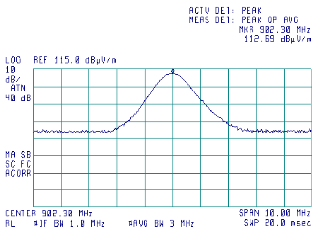
Plot 7.6.4 Field strength of carrier at low frequency
