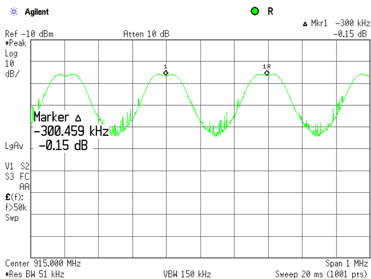
Plot 7.3.2 Carrier frequency separation
