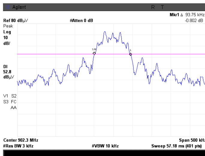
Plot 7.2.4 The 20 dB bandwidth test result at low frequency
