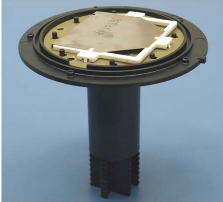
Photograph No.1 2WB-LG booster with cover removed
