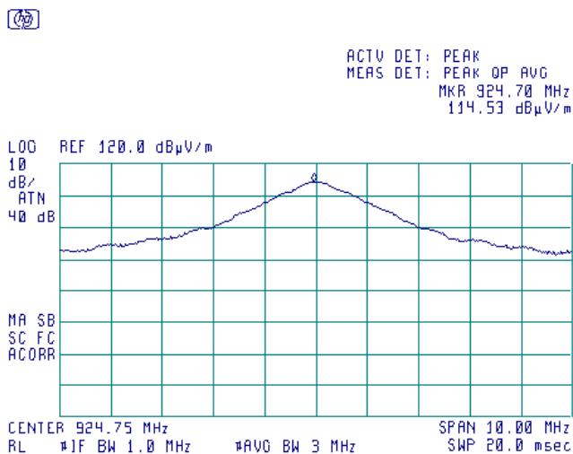
Plot 7.3.3 Field strength of carrier at high frequency
