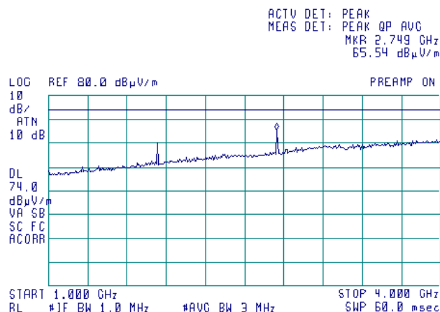
Plot 7.4.16 Radiated emission measurements from 1000 to 4000 MHz at the mid carrier frequency
