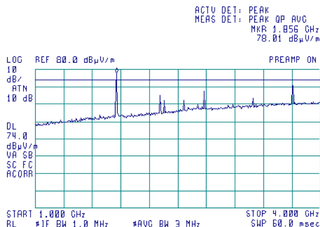
Plot 7.4.18 Radiated emission measurements from 1000 to 4000 MHz at the high carrier frequency
