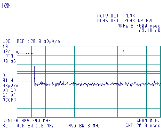
Plot 7.4.101 Transmission pulse duration, modulation PSK
