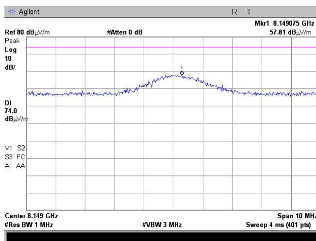
Plot 7.4.85 Radiated emission measurements at the ninth harmonic of low carrier frequency
