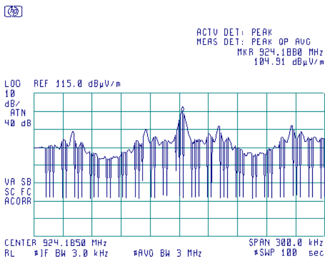
Plot 7.2.6 Peak spectral power density at high frequency zoomed at the peak, PSK modulation
