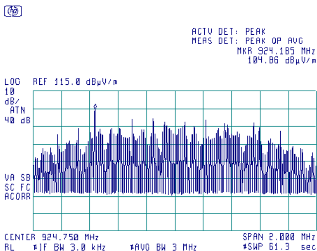
Plot 7.2.5 Peak spectral power density at high frequency within 6 dB band, PSK modulation
