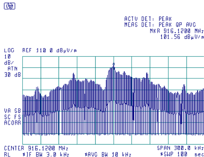
Plot 7.2.8 Peak spectral power density zoomed at the peak, FSK modulation
