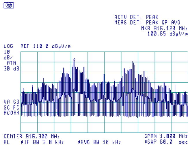
Plot 7.2.7 Peak spectral power density within 6 dB band, FSK modulation
