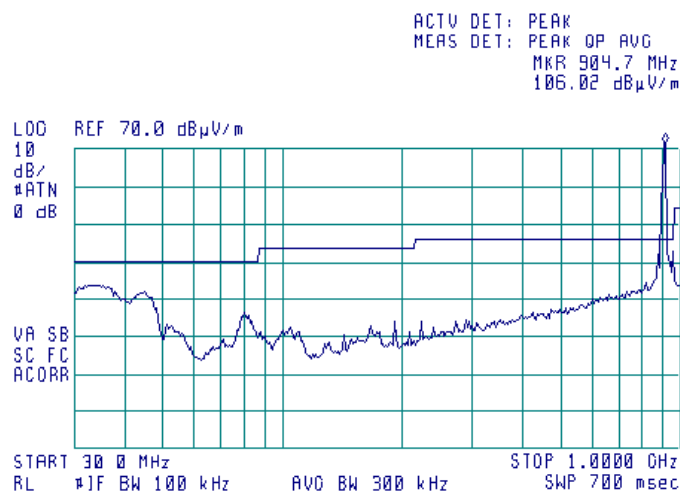
Plot 7.7.10 Radiated emission measurements from 30 to 1000 MHz at the mid carrier frequency
