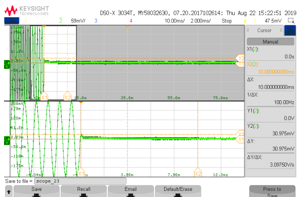
Plot 7.6.1 Transient frequency during power ON test results at low carrier frequency
