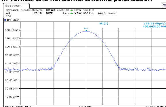
Plot 7.1.1 Transmitter carrier field strength at low frequency in vertical and horizontal antenna polarization
