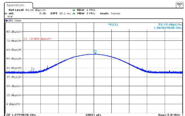
Plot 7.4.8 Radiated spurious emission measurements at the 5 th harmonic
