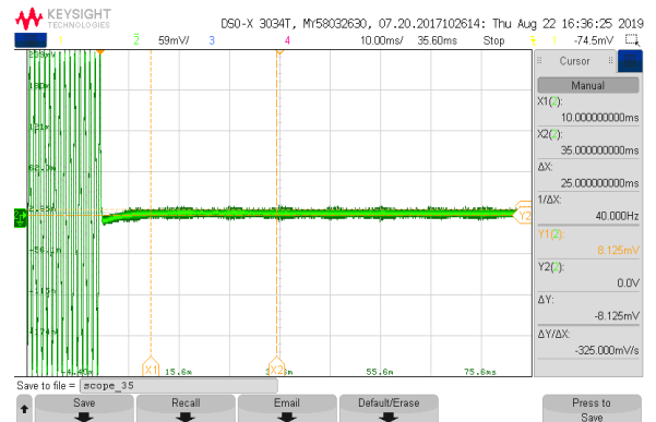
Plot 7.6.5 Transient frequency during power ON test results at high carrier frequency
