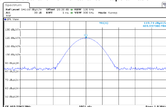
Plot 7.1.3 Transmitter carrier field strength at high frequency in vertical and horizontal antenna polarization
