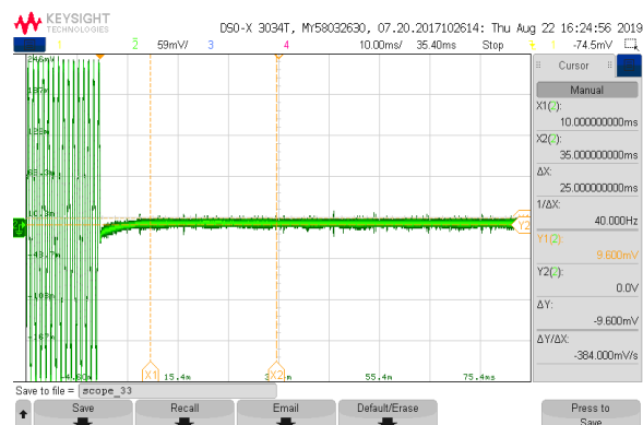
Plot 7.6.3 Transient frequency during power ON test results at mid carrier frequency
