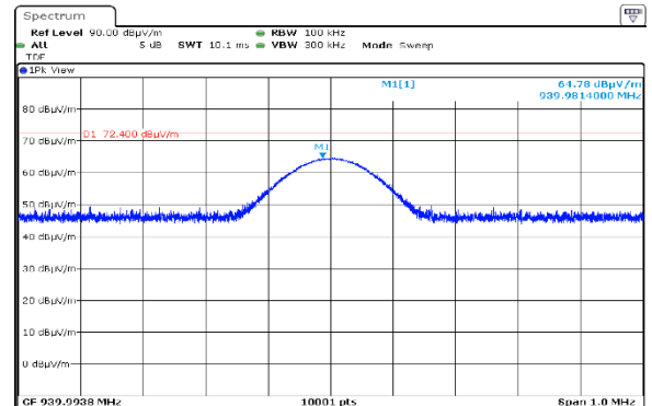
Plot 7.4.6 Radiated spurious emission measurements at the 3 rd harmonic
