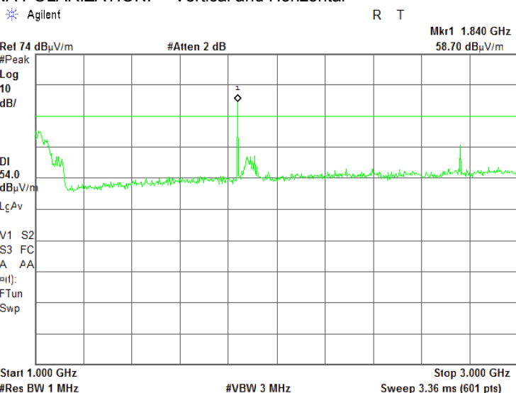
Plot 7.3.21 Radiated emission measurements from 1000 to 3000 MHz at the high carrier frequency
