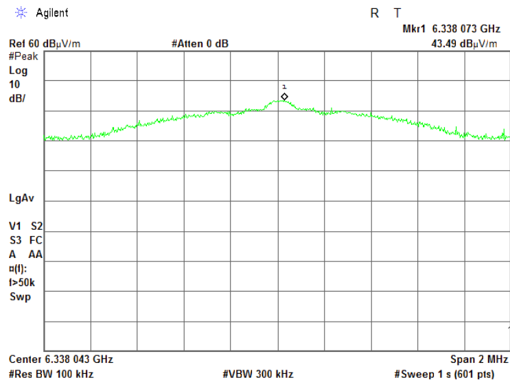
Plot 7.3.41 Radiated emission measurements at the eighth harmonic of low carrier frequency
