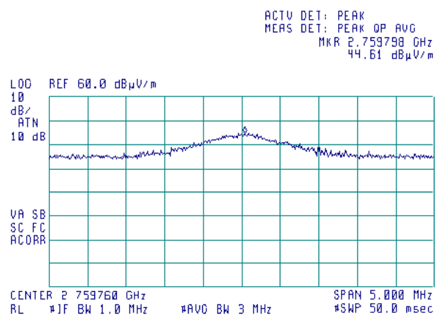
Plot 7.3.31 Radiated emission measurements at the third harmonic of high carrier frequency
