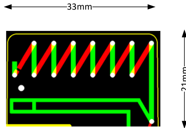
Printed antenna
