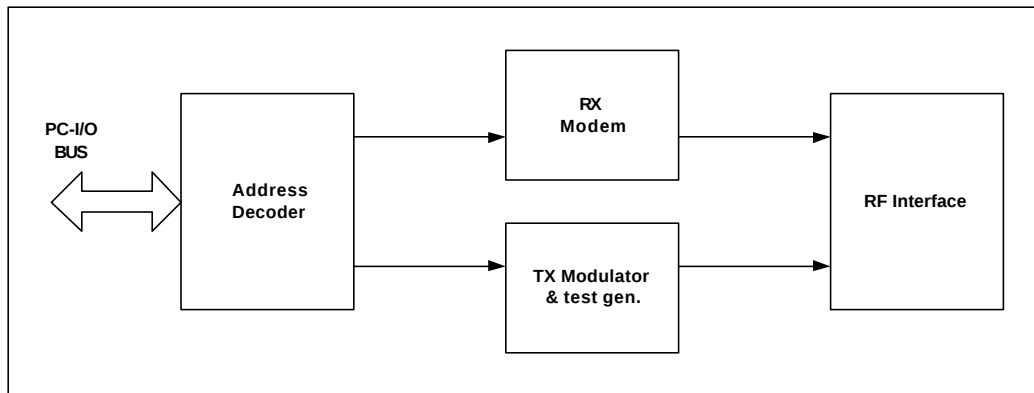
DMU Block Diagram
